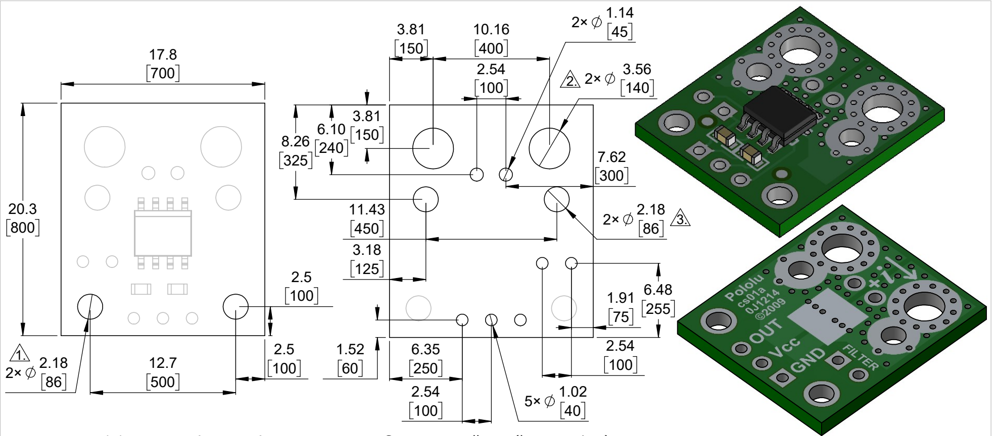
① Board dimensions (top view) Scale 3:1
