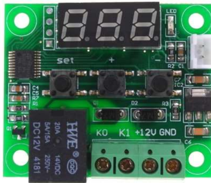
RELAY CONTACTS TO HEATER/COOLER
