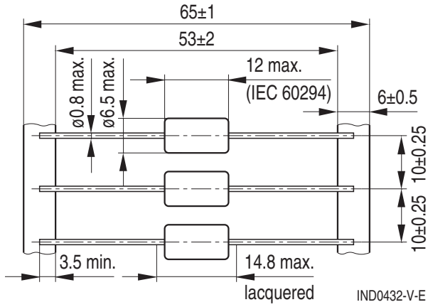
Dimensions in mm Minimum lead spacing 15 mm
