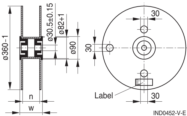
n (mm): 72 +1 w (mm): 84 max
