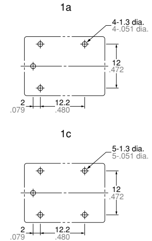
PC board pattern (Bottom view)
