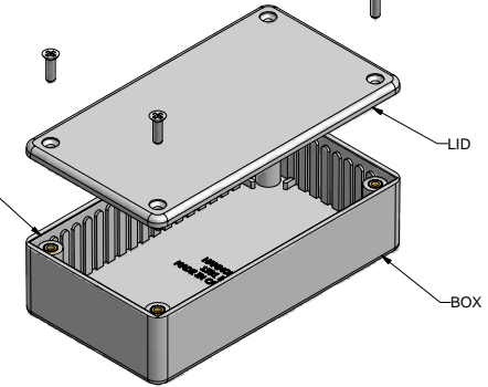
EXPLODED VIEW OF ENCLOSURE
