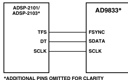
Figure 10. ADSP-2101/ADSP-2103 to AD9833 Interface
