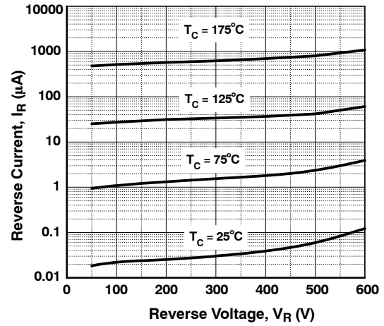
Figure 22. Reverse Current
