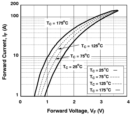
Figure 21. Forward Characteristics
