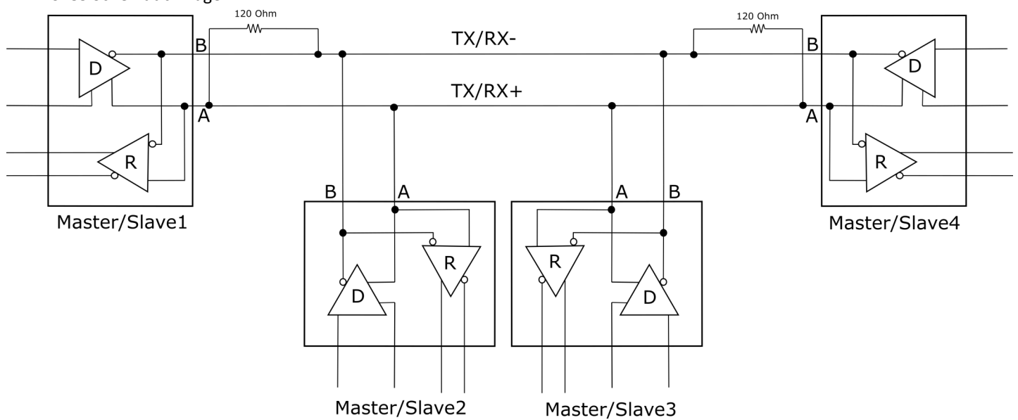
RS485 Schematic image:
