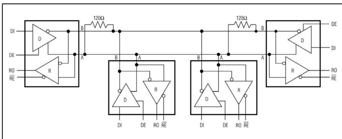
Figure 11: Typical half-duplex XD/XL485 operating network
