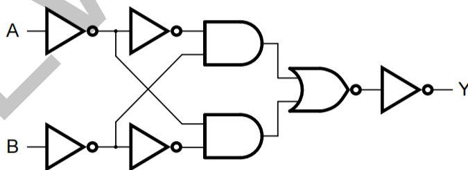
Figure 3. Logic diagram for one gate
