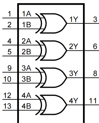
Figure 1. Logic symbol
