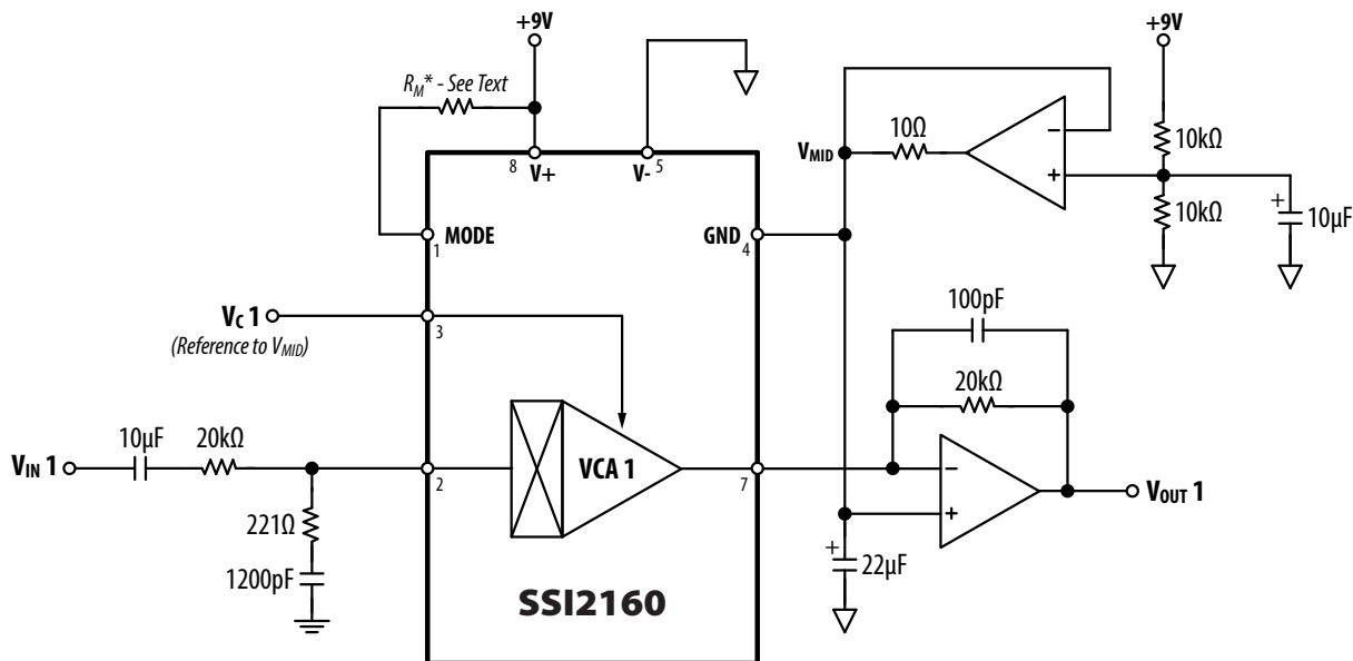
Figure 6: Single-Supply Operation
