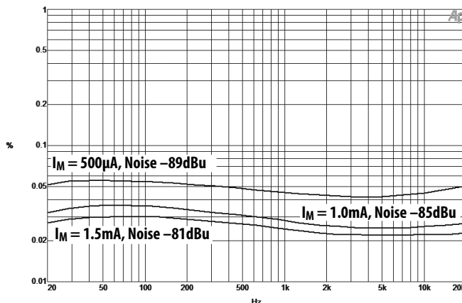
Figure 3: SSI2160 Class A THD+N At Varying Mode Currents
