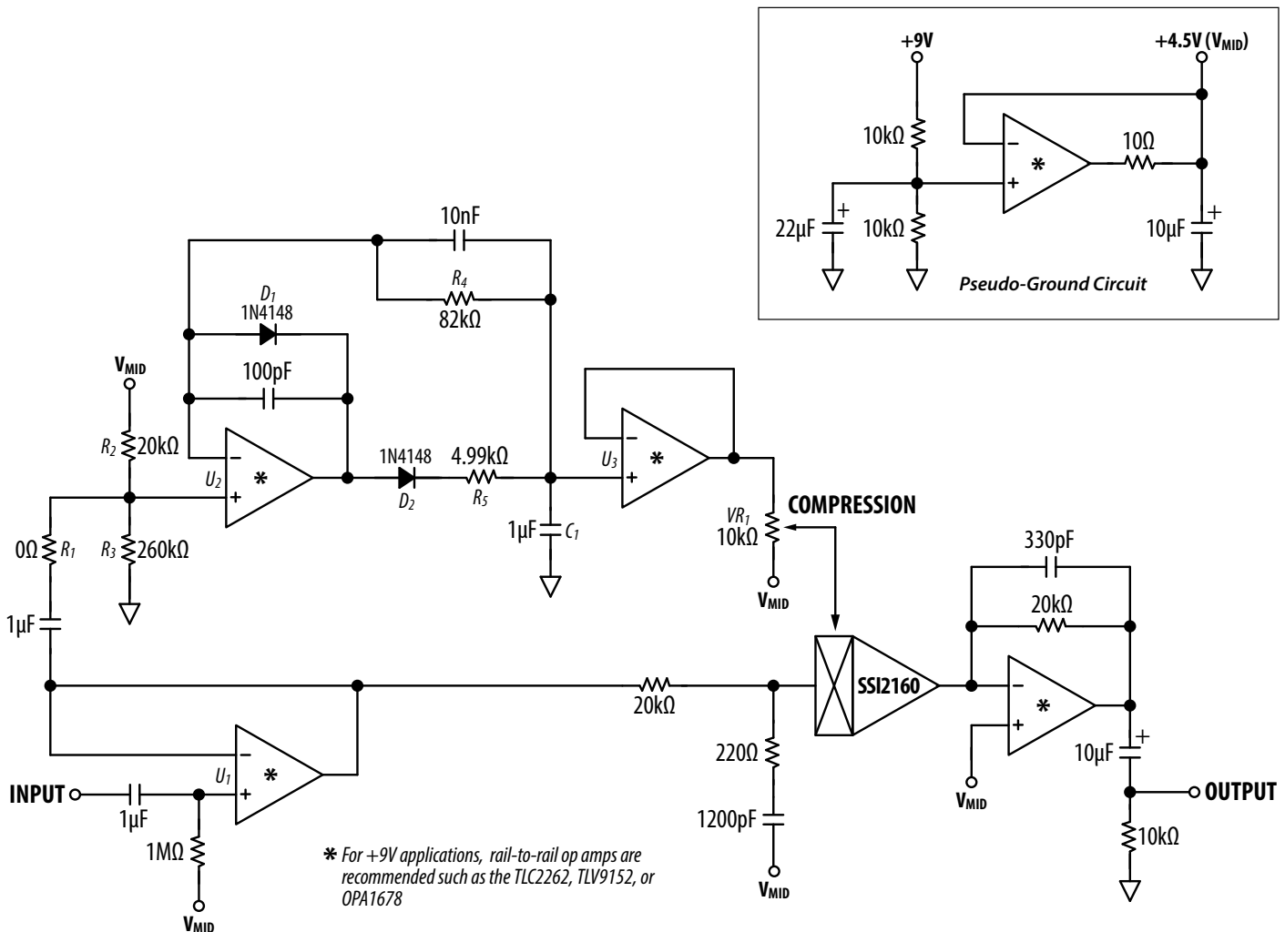
Figure 10: Compressor Modified for +9V Systems
