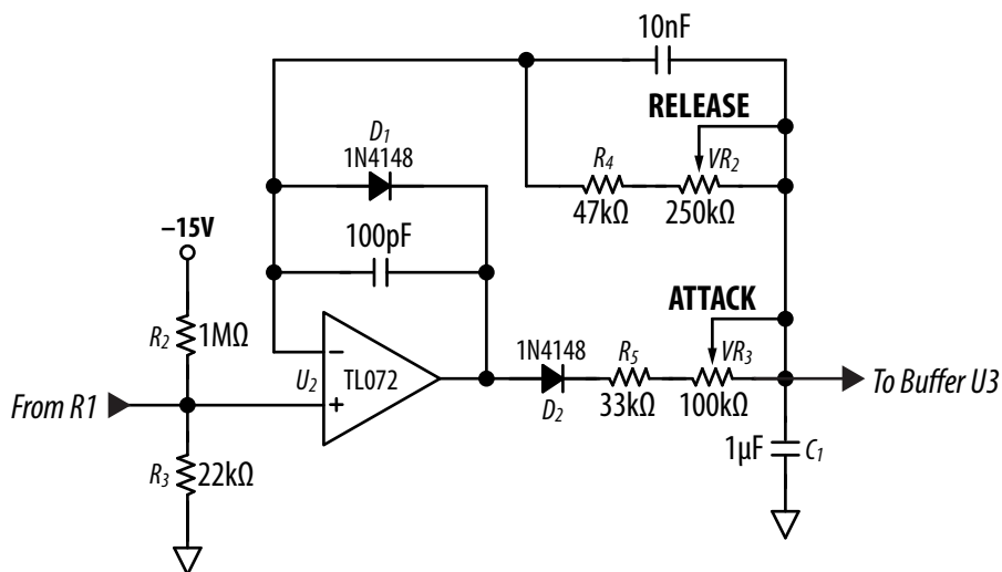
Figure 8: Envelope Detector with Attack and Release Controls
