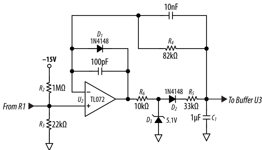
Figure 9: Envelope Detector with Voltage Clamp
