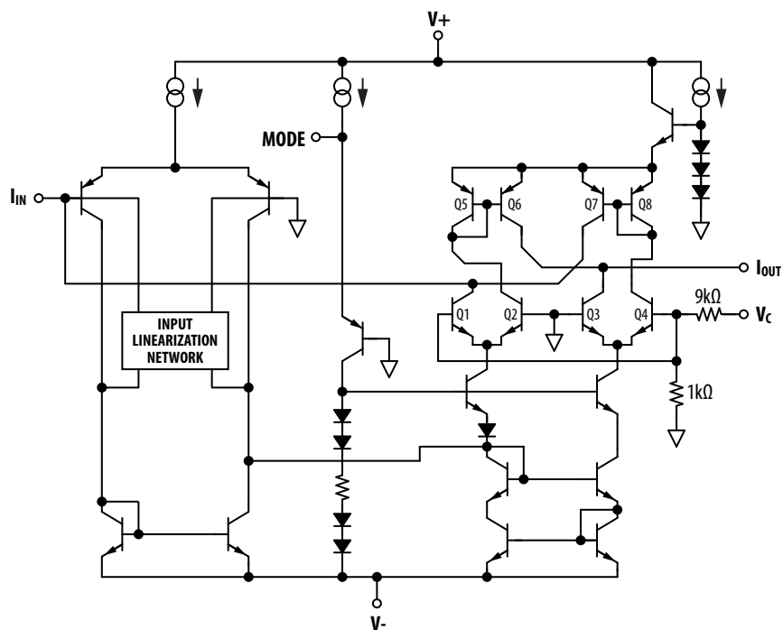
Figure 4: SSI2160 Simplified Schematic
