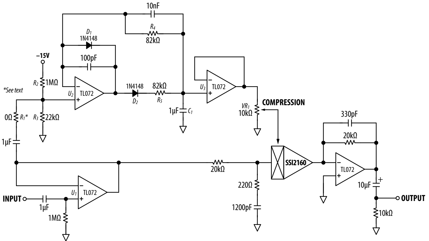
Figure 7: SSI2160-Based One-Knob Compressor
