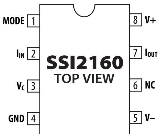
PIN CONNECTIONS 8-LEAD SOP
