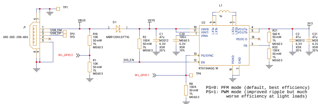
Figure 8. The powerchain of the Pico W Rev3 board
