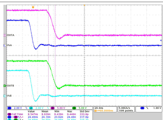
Figure 8-6. Falling Time and Turnoff Propagation Delay
