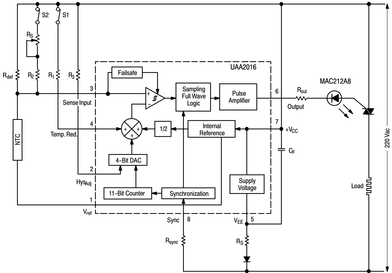
Figure 1. Application Schematic
