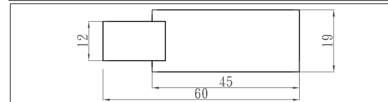
RECOMMENDED PCB SIZE
