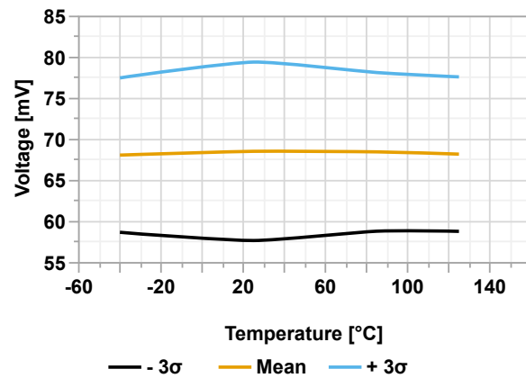
Figure 46-47. BOR Hysteresis (BORV[1:0] = 1) vs. Temperature
