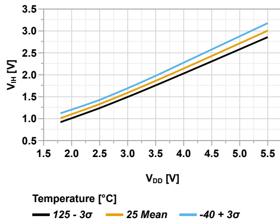
Figure 46-59. Input Pin with Schmitt Trigger - Minimum V_{IH} vs. V_{DD}
