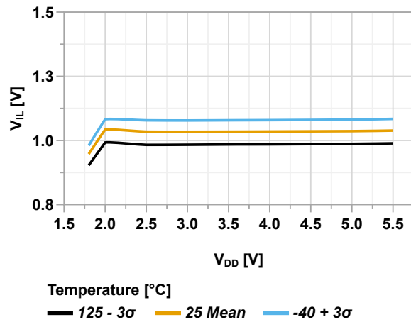
Figure 46-61. Input Pin with LVBUF - Maximum V_{IL} vs. V_{DD}
