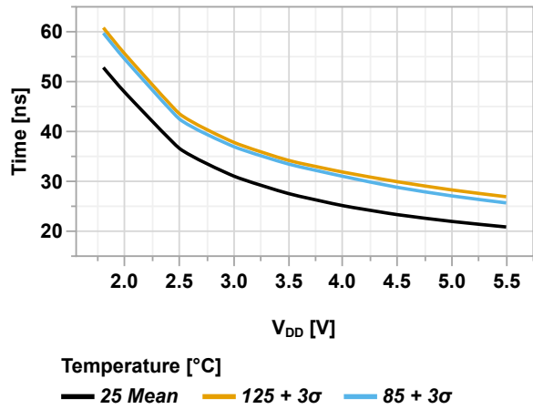
Figure 46-56. Rise Time (SLRxn = b ' 1) vs. V_{DD}
