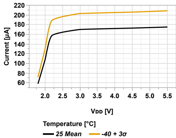
Figure 46-16. I_{PD} Base (VREGPM[1:0] = 'b00 = HP) vs. V_{DD}
