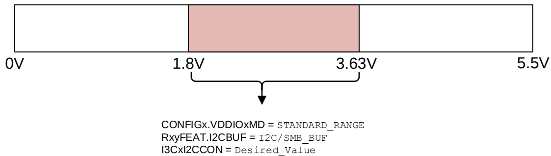
Figure 37-4. Pad Buffer Selection for I2C Mode Operation
