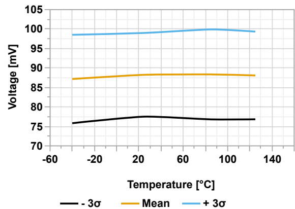
Figure 46-49. BOR Hysteresis (BORV[1:0] = 3) vs. Temperature
