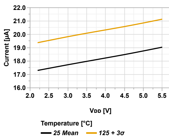
Figure 46-24. I_{PD} HLVD vs. V_{DD}
