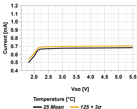
Figure 46-12. Doze Power Consumption vs. V_{DD} (RSTOSC[2:0] = 'b110, OSCFRQ = 16 MHz, PMDx = 0xFF)
