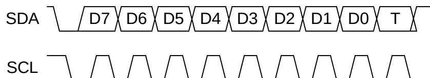
Figure 37-12. I3C® Data Word in Push-Pull Bus Configuration
