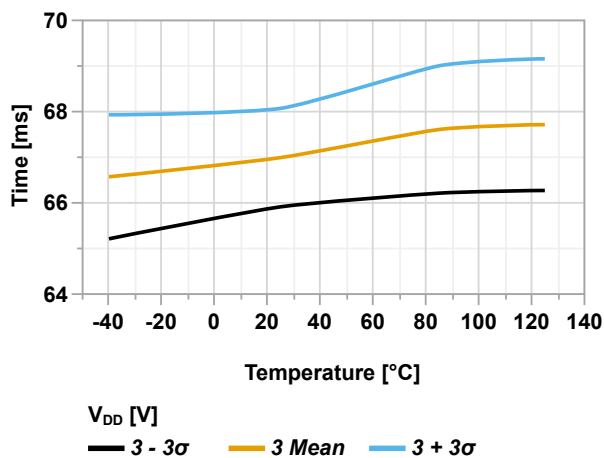
Figure 46-38. Start-up Time vs. Temperature (PWRTS[1:0] = 0x2, V_{DD} = 3.0V)
