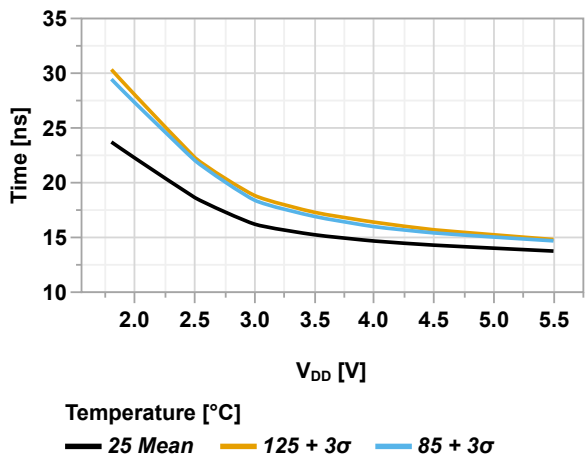
Figure 46-57. Rise Time (SLRxn = b ' 0) vs. V_{DD}
