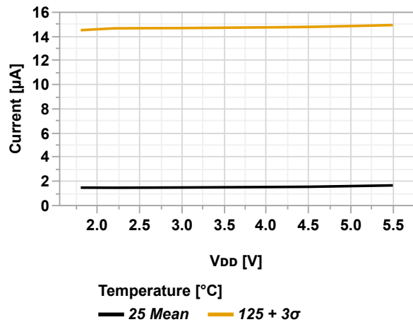
Figure 46-14. I_{PD} Base (VREGPM[1:0] = 'b10 = ULP) vs. V_{DD}
