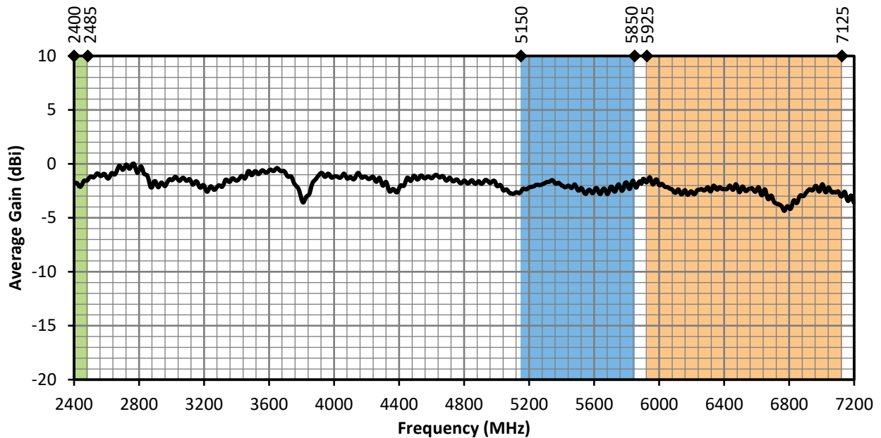
Figure 7. ANT-W63WS5-ccc Antenna Average Gain, Straight
