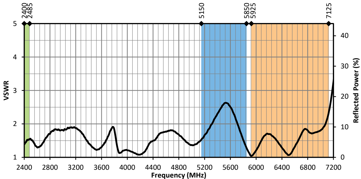
Figure 11. ANT-W63WS5-ccc VSWR, Edge-Bent
