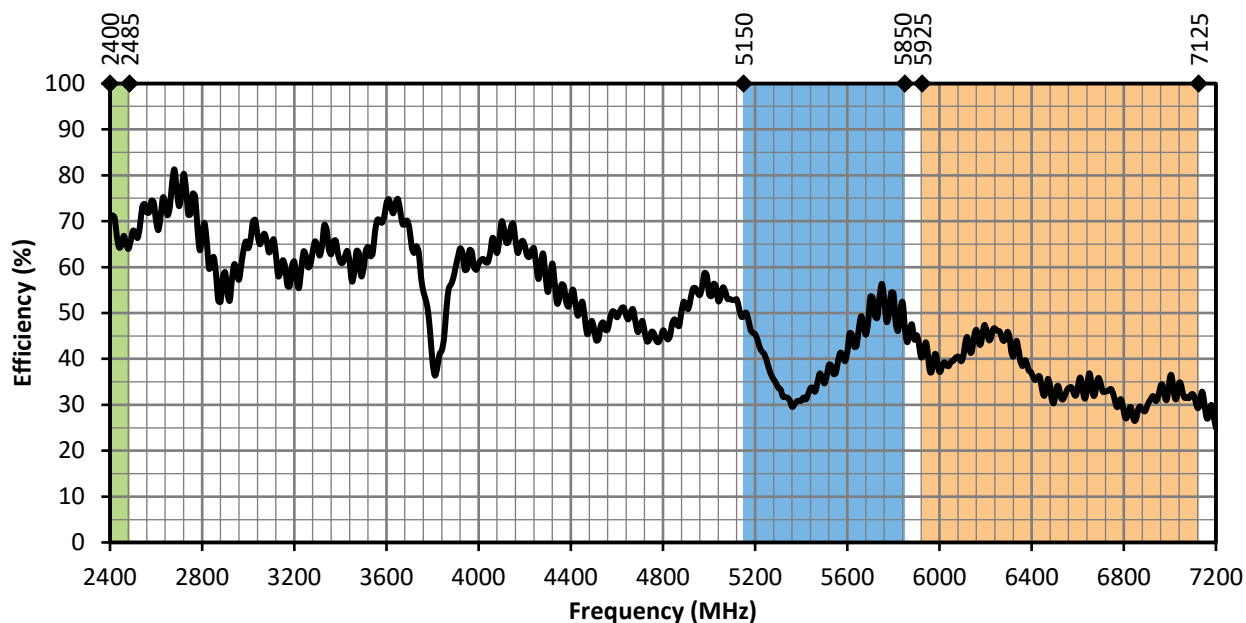
Figure 15. ANT-W63WS5-ccc Antenna Efficiency, Edge-Bent
