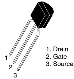
TO-92 3 LF CASE 135AR
