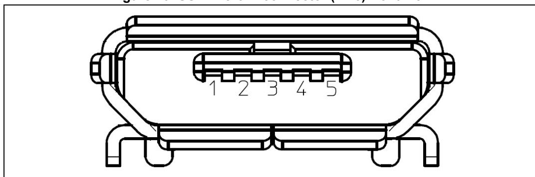
Figure 15. USB Micro-B connector (CN5) front view
