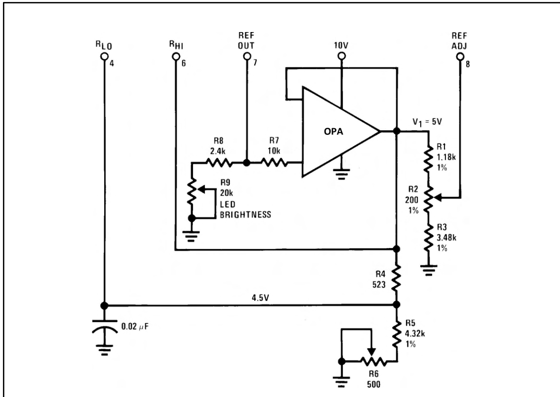
Figure 10-2. Non-Interacting Adjustments for Expanded Scale Meter
