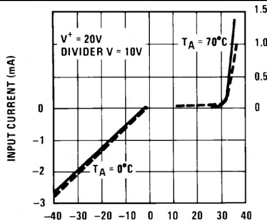
Figure 7-7. Input Current Beyond Signal Range (Pin 5)
