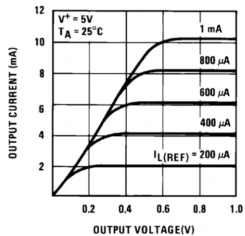
Figure 7-12. Output Characteristics
