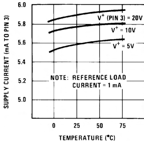
Figure 7-1. Supply Current vs Temperature
