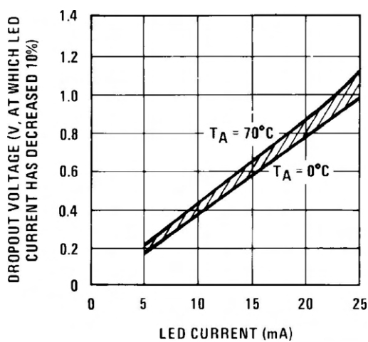
Figure 7-5. LED Current-Regulation Dropout
