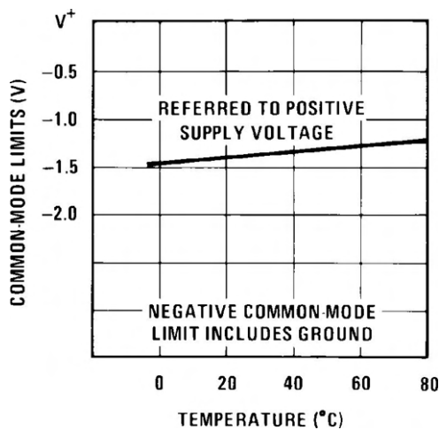
Figure 7-11. Common-Mode Limits
