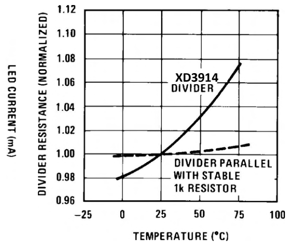
Figure 7-10. Total Divider Resistance vs Temperature
