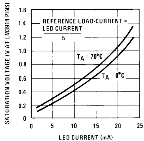
Figure 7-6. LED Driver Saturation Voltage
