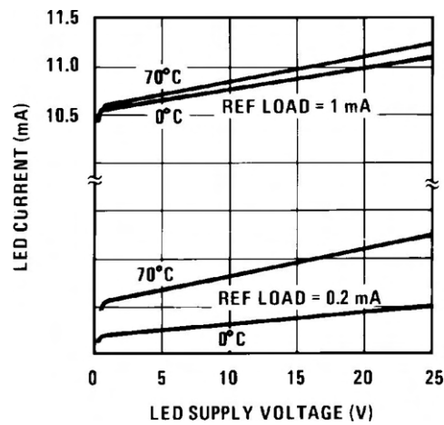
Figure 7-9. LED Driver Current Regulation
