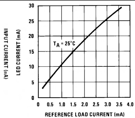
Figure 7-8. LED Current vs Reference Loading
