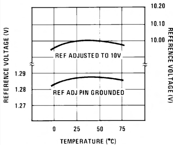
Figure 7-3. Reference Voltage vs Temperature
