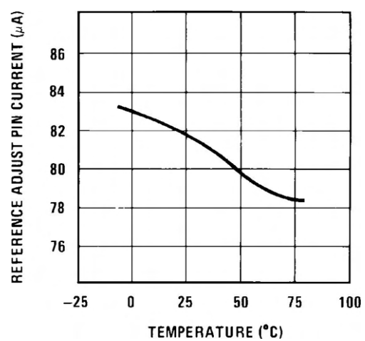
Figure 7-4. Reference Adjust Pin Current vs Temperature
