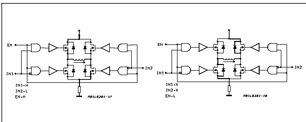
Figure 8c: Enable Chopping
