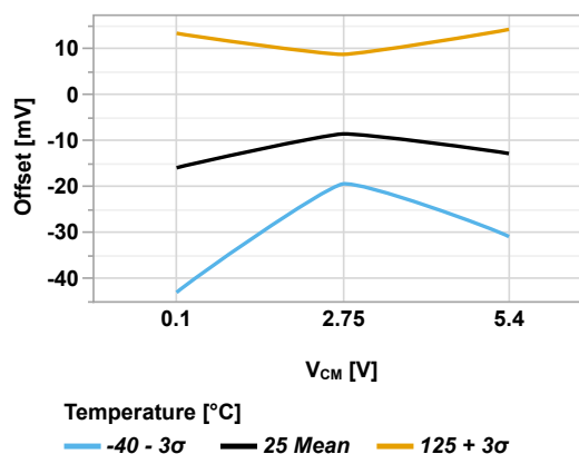
Figure 45-162. Input Offset vs Common-Mode Voltage ( V_{DD} = 5.5V )
