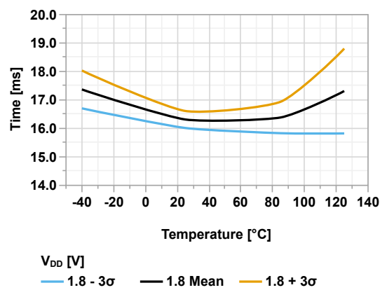
Figure 45-89. WDT Time-out Period vs Temperature ( V_{DD} = 1.8V )
