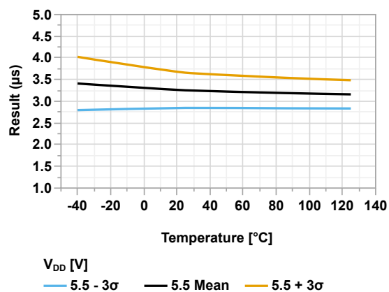
Figure 45-119. DAC Settling Time vs. Temperature ( V_{DD} = 5.5V )
