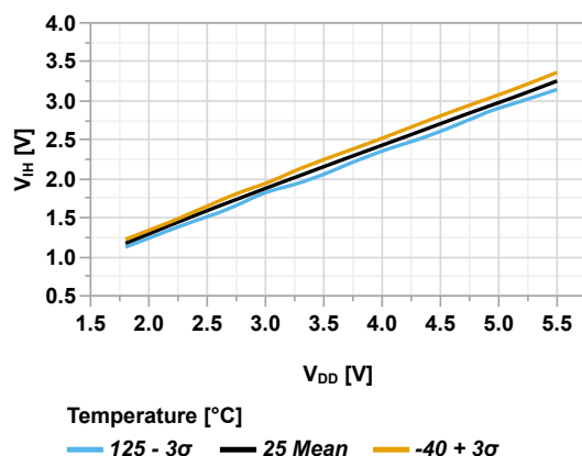
Figure 45-58. Input Pin with I 2 C Trigger Minimum V_{IH} vs V_{DD}
