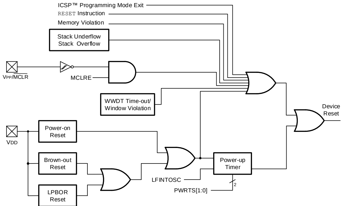
Figure 10-1. Simplified Block Diagram of On-Chip Reset Circuit
