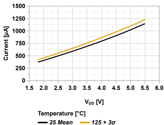
Figure 45-17. I_{DD} vs V_{DD} (XT = 4 MHz, PMDx = 0x00)
