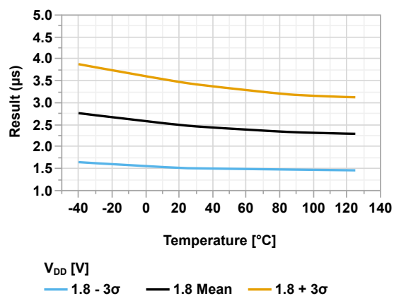
Figure 45-117. DAC Settling Time vs. Temperature ( V_{DD} = 1.8V )
