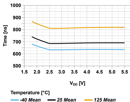
Figure 45-193. ZCD Falling-Edge Response Time vs V_{DD} (Mean Values)
