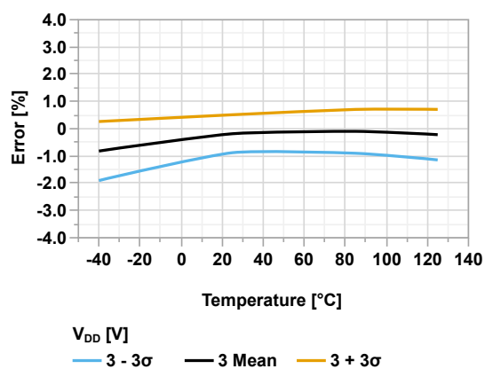
Figure 45-173. ADFVR Voltage Error vs Temperature ( V_{DD} = 3.0\text{V} , V_{REF} = 1.024\text{V} )
