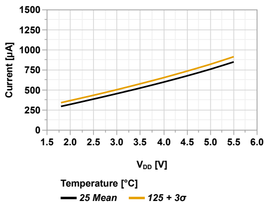
Figure 45-18. I_{DD} vs V_{DD} (XT = 4 MHz, PMDx = 0xFF)
