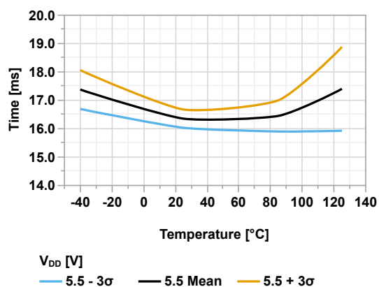
Figure 45-91. WDT Time-out Period vs Temperature ( V_{DD} = 5.5V )
