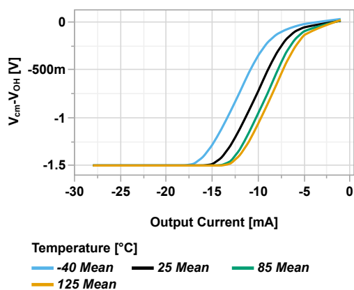
Figure 45-150. V_{OH} vs Temperature and Load Current ( V_{DD} = 5.5V )
