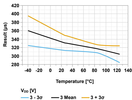
Figure 45-73. LFO Oscillator Start-Up Time vs Temperature ( V_{DD} = 3.0V )
