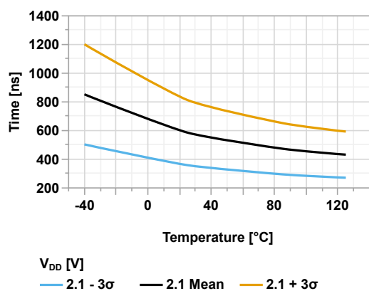
Figure 45-83. BOR Minimum Pulse Width for Response vs Temperature
