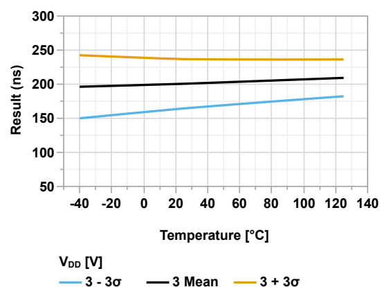
Figure 45-169. Falling Edge Response Time vs Temperature (CxSP = '1', CPON = 'b01', V_{DD} = 3.0V)
