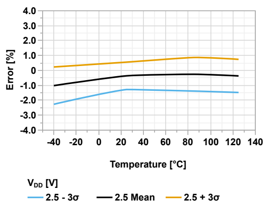
Figure 45-172. ADFVR Voltage Error vs Temperature ( V_{DD} = 2.5\text{V} , V_{REF} = 1.024\text{V} )
