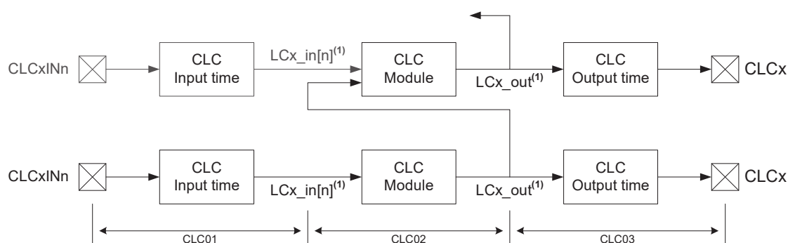
Figure 44-21. CLC Propagation Timing
