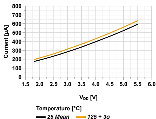
Figure 45-4. I_{DD} vs V_{DD} (HFINTOSC = 2 MHz, PMDx = 0xFF)
