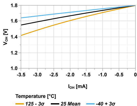
Figure 45-60. Output Pin Minimum V_{OH} vs Current ( V_{DD} = 1.8V )
