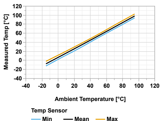
Figure 45-185. TEMPERATURE INDICATOR CHARACTERISTICS ( V_{DD} = 3.0V )
