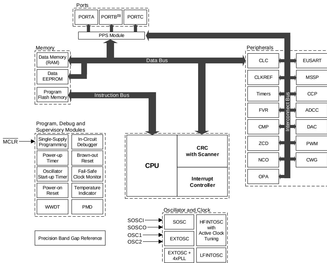
Figure 1. PIC16F17126/46 Block Diagram
