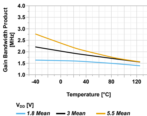
Figure 45-127. Gain Bandwidth Product vs Temperature (CPON = '0', GSEL = 'b001')
