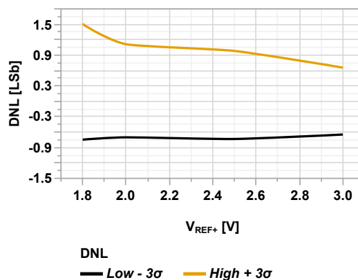
Figure 45-96. ADC DNL vs V_{REF+} (Single-Ended Mode, T_{AD} = 1 \mu s , V_{DD} = 3.0V , T_A = 125^\circ C , CPON = 'b11')
