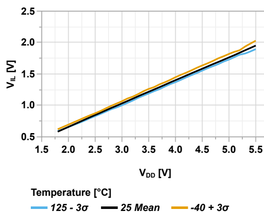
Figure 45-53. Input Pin with Schmitt Trigger Maximum V_{IL} vs V_{DD}
