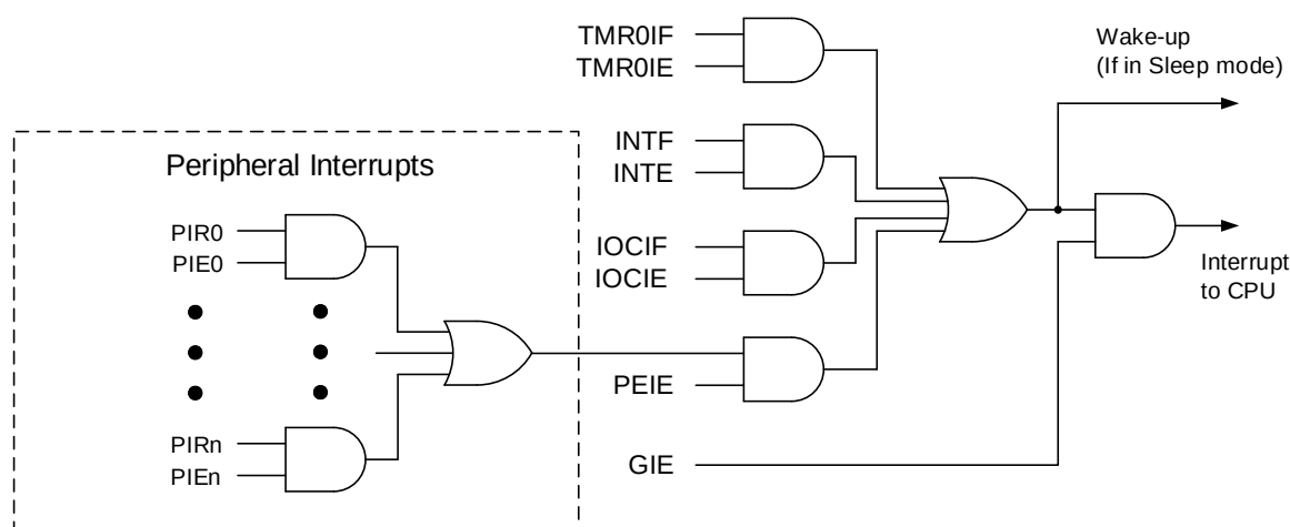
Figure 12-1. Interrupt Logic
