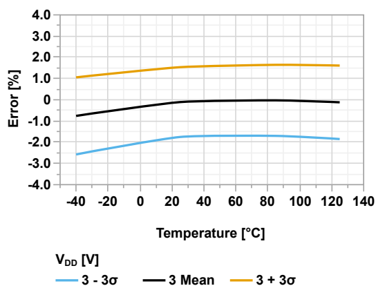
Figure 45-180. CDAFVR Voltage Error vs Temperature ( V_{DD} = 3.0V , V_{REF} = 1.024V )
