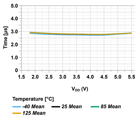
Figure 45-143. Slew Rate (Falling) vs V_{DD} and Temperature
