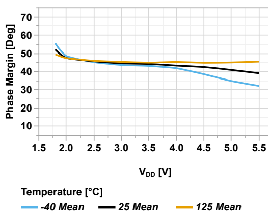
Figure 45-139. Phase Margin vs V_{DD} (CPON = '0', GSEL = 'b001')
