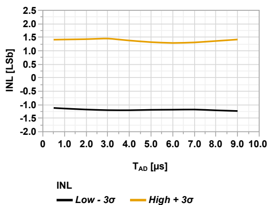
Figure 45-99. ADC INL vs T_{AD} (Single-Ended Mode, V_{REF+} = V_{DD} = 3.0V , T_A = 125^\circ C , CPON = 'b11')
