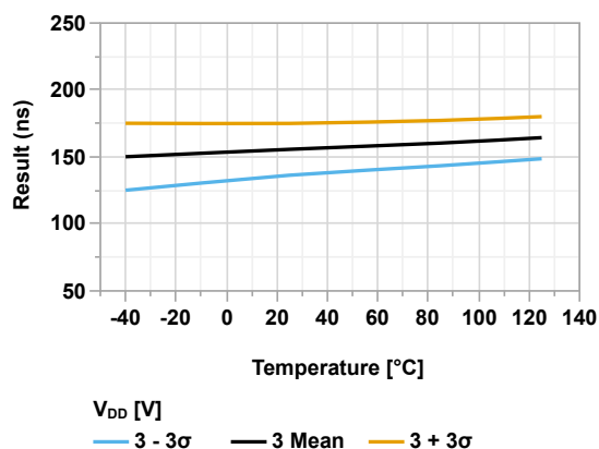
Figure 45-165. Rising Edge Response Time vs Temperature (CxSP = '1', CPON = 'b01', V_{DD} = 3.0V)
