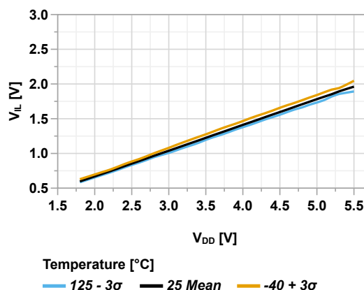
Figure 45-59. Input Pin with I 2 C Trigger Maximum V_{IL} vs V_{DD}
