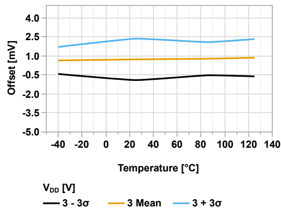
Figure 45-154. Offset vs Temperature ( V_{DD} = 3.0V , V_{CM} = V_{DD}/2 , Factory-Calibrated Input Offset Voltage)
