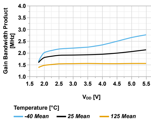
Figure 45-131. Gain Bandwidth Product vs V_{DD} (CPON = '0', GSEL = 'b001')
