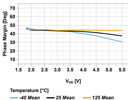
Figure 45-138. Phase Margin vs V_{DD} (CPON = '1', GSEL = 'b001')
