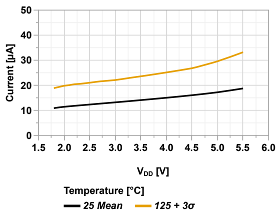
Figure 45-15. I_{DD} vs V_{DD} (XT = 1 MHz, PMDx = 0x00)
