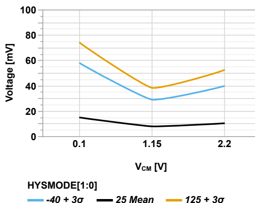
Figure 45-158. Input Hysteresis vs Common-Mode Voltage ( V_{DD} = 5.5V )
