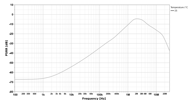
Figure 45-123. OPA PSRR (log(f) vs PSRR (dB) (Typical))
