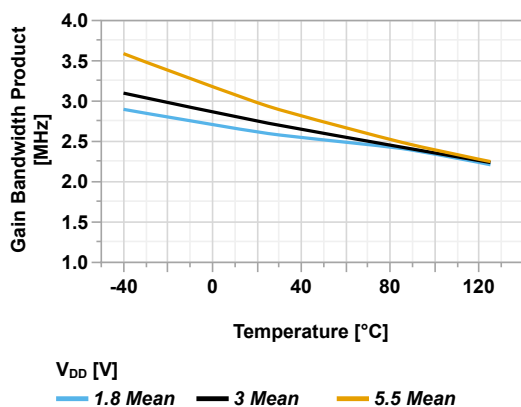
Figure 45-126. Gain Bandwidth Product vs Temperature (CPON = '1', GSEL = 'b001')
