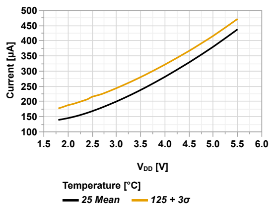
Figure 45-44. I_{PD} Op Amp (CPON = 'b00) vs V_{DD}
