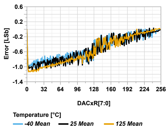
Figure 45-110. DAC INL vs. DAC Code ( V_{REF} = V_{DD} = 2.3V )
