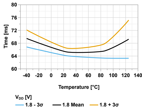
Figure 45-86. Start-Up Time vs Temperature (PWRTS = 'b10, VDD = 1.8V)
