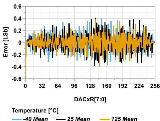
Figure 45-108. DAC DNL vs. DAC Code ( V_{REF} = V_{DD} = 5.5V )
