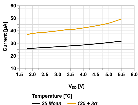
Figure 45-40. I_{PD} ADC (Not-converting) vs V_{DD}
