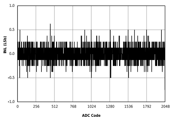
Figure 45-97. ADC INL vs ADC Code (Single-Ended Mode, V_{DD} = 3.0V , T_{AD} = 1 \mu s )
