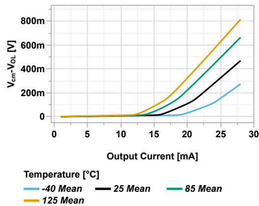
Figure 45-153. V_{OL} vs Temperature and Load Current ( V_{DD} = 5.5V )
