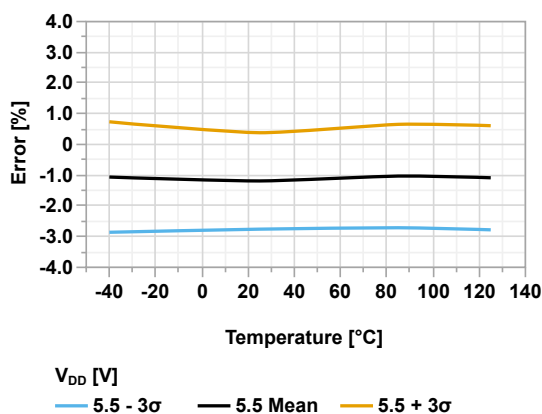
Figure 45-181. CDAFVR Voltage Error vs Temperature ( V_{DD} = 5.5V , V_{REF} = 1.024V )
