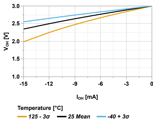
Figure 45-61. Output Pin Minimum V_{OH} vs Current ( V_{DD} = 3.0V )
