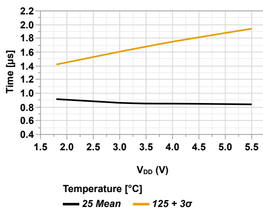
Figure 45-146. Turn-On Time vs V_{DD} and Temperature (CPON = '0')
