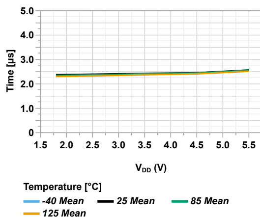
Figure 45-142. Slew Rate (Rising) vs V_{DD} and Temperature
