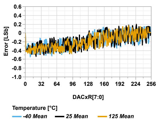
Figure 45-114. DAC INL vs. Temperature ( V_{REF} = V_{DD} = 3.0V )
