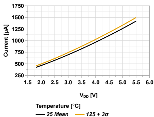
Figure 45-7. I_{DD} vs V_{DD} (HFINTOSC = 8 MHz, PMDx = 0x00)
