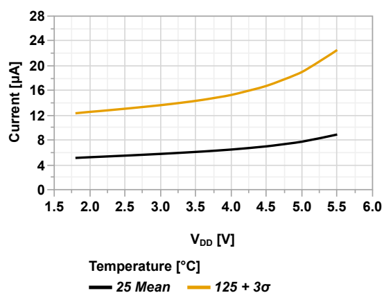
Figure 45-36. I_{PD} SOSC (High-Power Mode) vs V_{DD}
