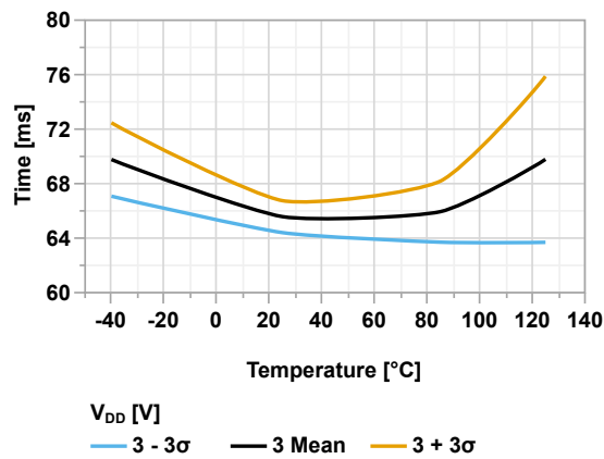
Figure 45-87. Start-Up Time vs Temperature (PWRTS = 'b10, VDD = 3.0V)
