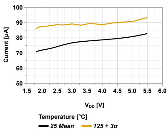
Figure 45-39. I_{PD} Comparator (High-Power Mode) vs V_{DD}
