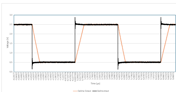
Figure 45-120. OPA Large Signal
