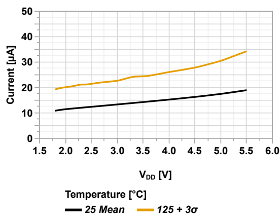
Figure 45-23. I_{DD} vs V_{DD} (ECL = 500 kHz, PMDx = 0x00)
