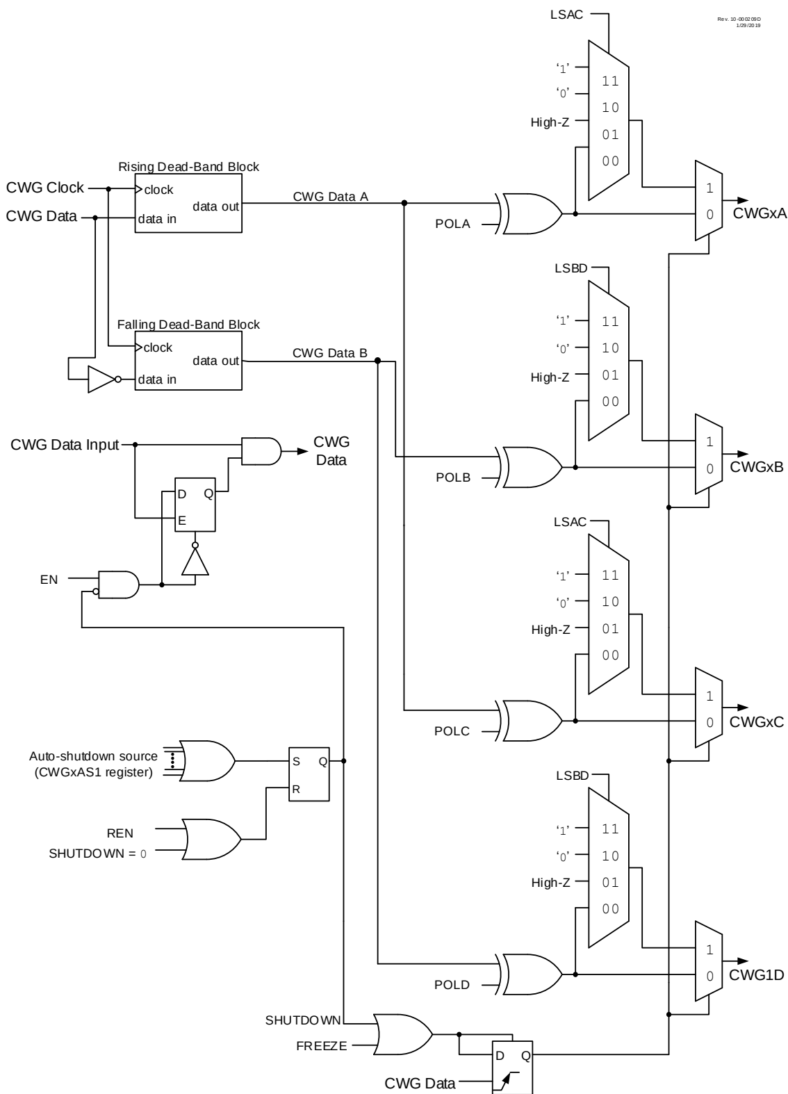
Figure 26-2. Simplified CWG Block Diagram (Half Bridge Mode, MODE = 'b100)
