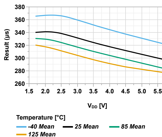
Figure 45-75. LFO Oscillator Start-Up Time vs V_{DD}
