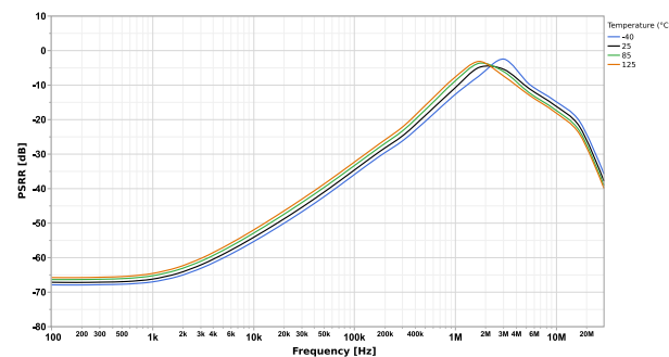
Figure 45-122. OPA PSRR (log(f) vs PSRR (dB) over Temperature)
