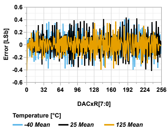
Figure 45-107. DAC DNL vs. DAC Code ( V_{REF} = V_{DD} = 5.0V )
