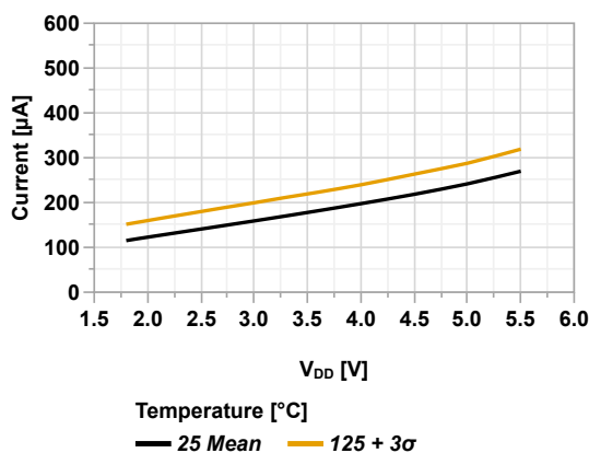
Figure 45-18. I_{DD} vs V_{DD} (XT = 4 MHz, PMDx = 0xFF)
