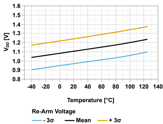
Figure 45-85. POR Rearm Voltage vs Temperature
