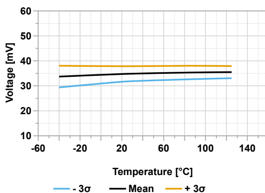
Figure 45-80. Brown-out Reset Hysteresis vs Temperature (BORV = '0')
