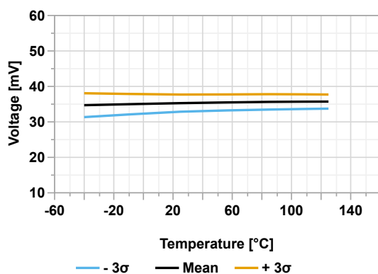
Figure 45-79. Brown-out Reset Hysteresis vs Temperature (BORV = '1')
