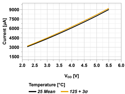
Figure 45-11. I_{DD} vs V_{DD} (HFINTOSC = 32 MHz, PMDx = 0x00)
