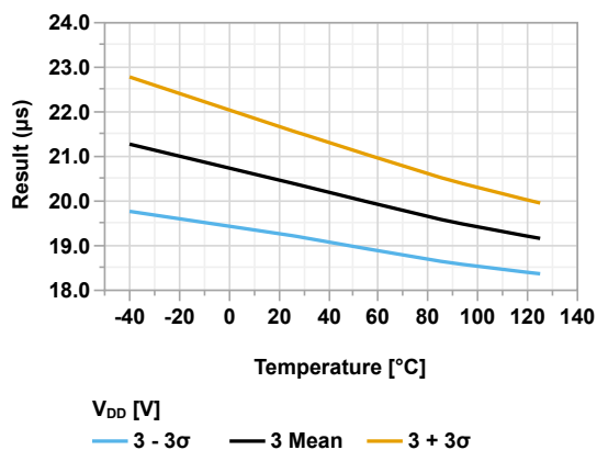
Figure 45-69. HFO Oscillator Start-Up Time vs Temperature ( V_{DD} = 3.0V )
