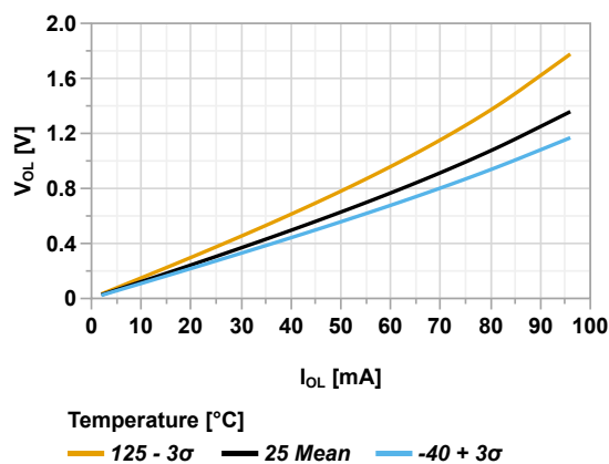
Figure 45-65. Output Pin Maximum V_{OL} vs Current ( V_{DD} = 5.5V )
