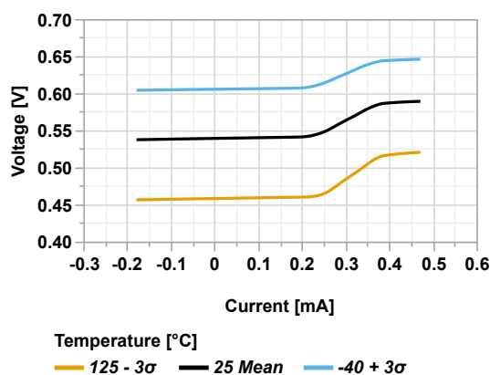
Figure 45-186. ZCD Pin Voltage vs Current, ( V_{DD} = 1.8V )
