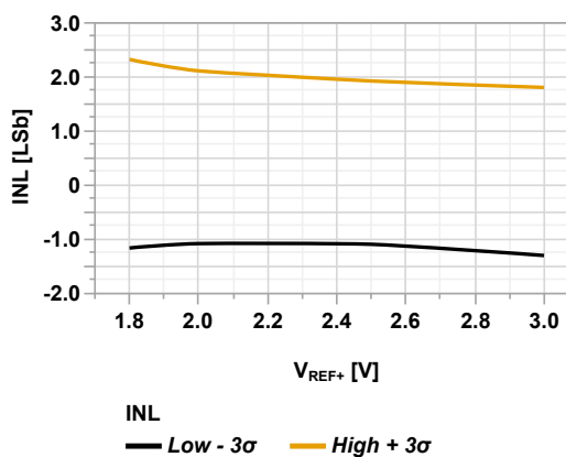
Figure 45-100. ADC INL vs V_{REF+} (Single-Ended Mode, T_{AD} = 1 \mu s , V_{DD} = 3.0V , T_A = 125^\circ C , CPON = 'b11')
