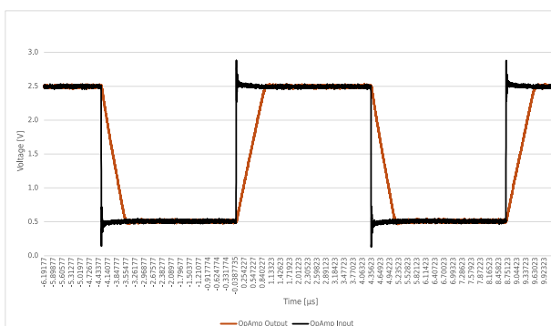
Figure 45-121. OPA Small Signal
