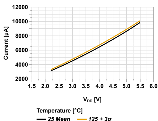
Figure 45-21. I_{DD} vs V_{DD} (ECL = 32 kHz, PMDx = 0x00)
