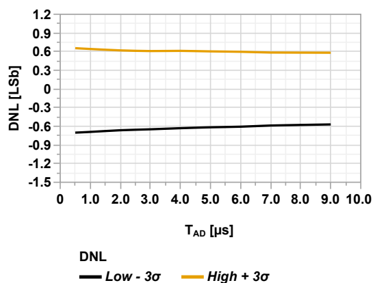
Figure 45-95. ADC DNL vs T_{AD} (Single-Ended Mode, V_{REF+} = V_{DD} = 3.0V , T_A = 125^\circ C , CPON = 'b11')
