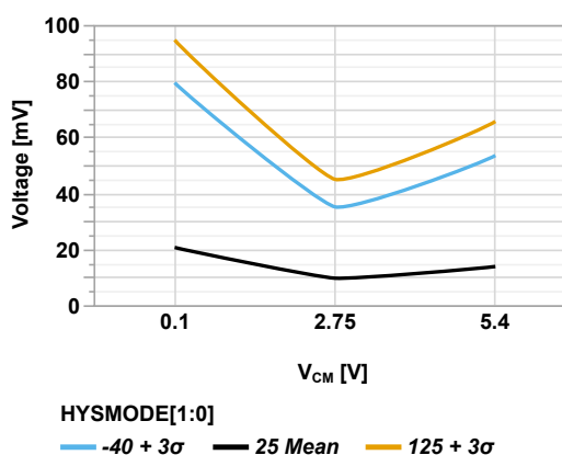
Figure 45-158. Input Hysteresis vs Common-Mode Voltage ( V_{DD} = 5.5V )
