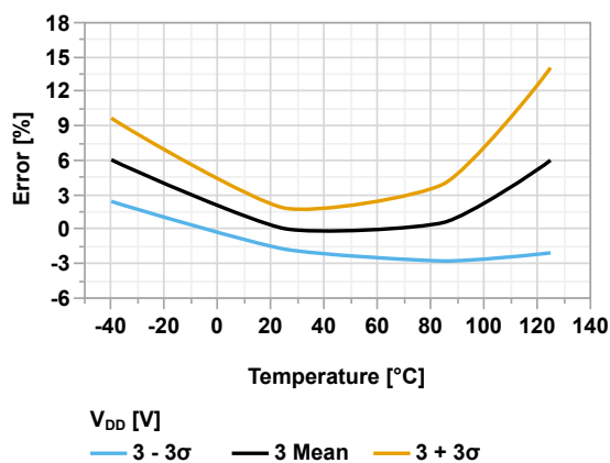
Figure 45-76. LFO Oscillator Error (%) vs Temperature ( V_{DD} = 3.0V )
