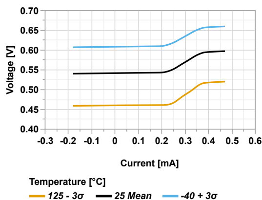
Figure 45-187. ZCD Pin Voltage vs Current, ( V_{DD} = 2.0V )
