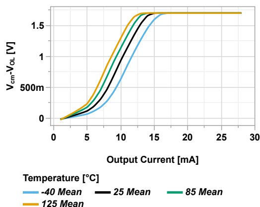
Figure 45-151. V_{OL} vs Temperature and Load Current ( V_{DD} = 2.0V )
