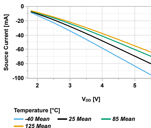
Figure 45-141. Source Current vs Temperature
