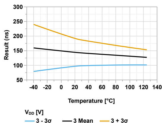
Figure 45-170. Falling Edge Response Time vs Temperature (CxSP = '0', CPON = 'b01', V_{DD} = 3.0V)
