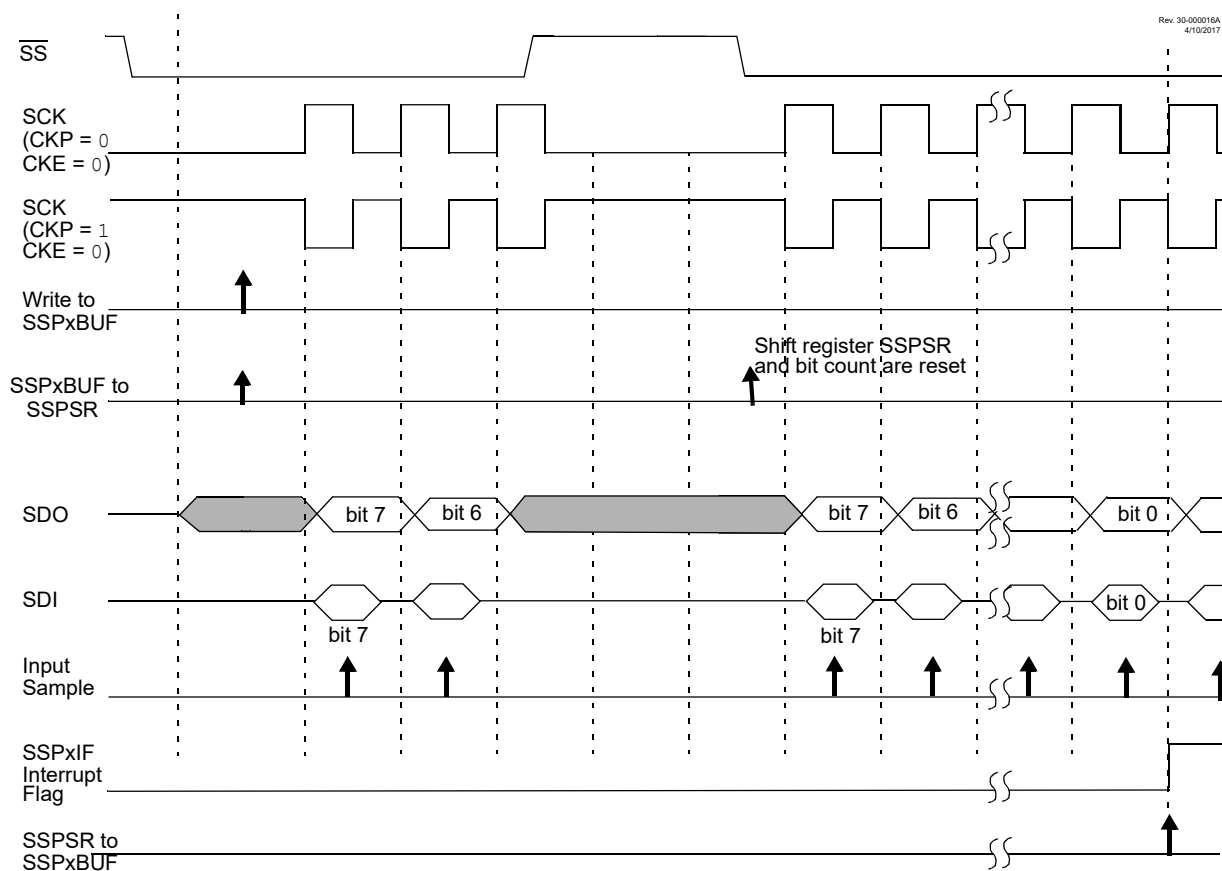
Figure 31-6. Client Select Synchronous Waveform
