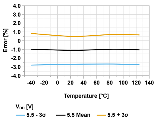
Figure 45-183. CDAFVR Voltage Error vs Temperature ( V_{DD} = 5.5V , V_{REF} = 2.048V )
