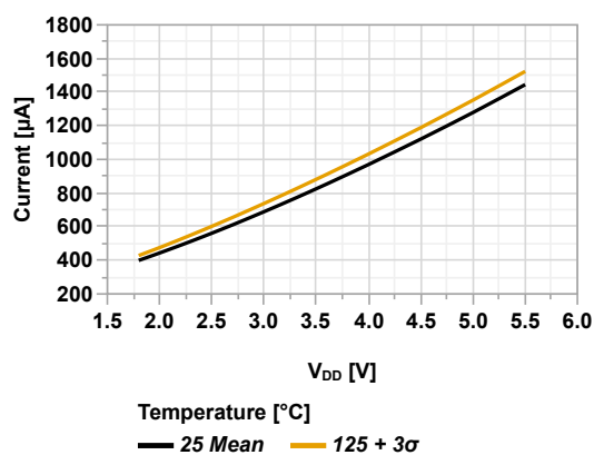
Figure 45-30. I_{DD} vs V_{DD} (Idle Mode, HFINTOSC = 16 MHz, PMDx = 0xFF)
