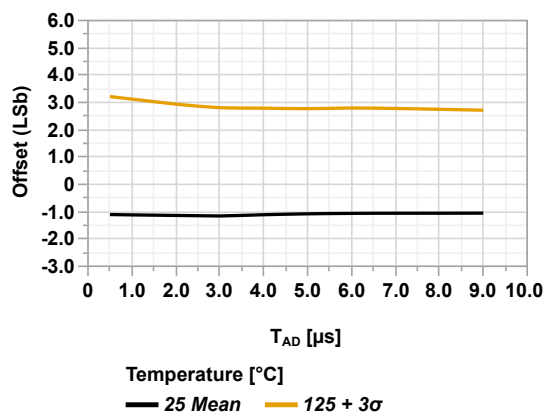
Figure 45-103. ADC Offset Error vs T_{AD} (Single-Ended Mode, V_{REF+} = V_{DD} = 3.0V , CPON = 'b11')
