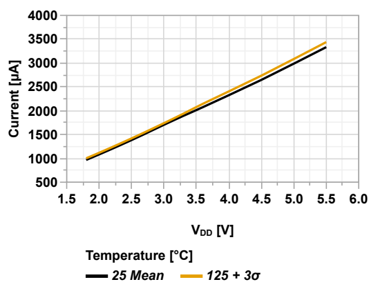
Figure 45-12. I_{DD} vs V_{DD} (HFINTOSC = 32 MHz, PMDx = 0xFF)
