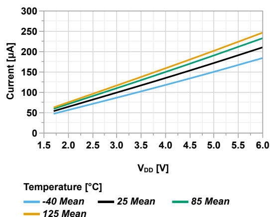
Figure 45-67. Weak Pull-Up Current vs V_{DD} (Mean Values)
