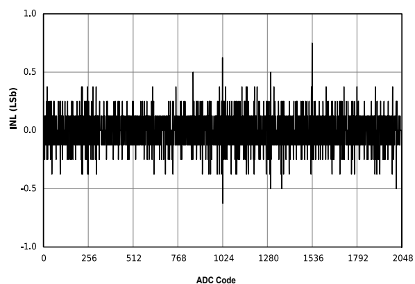
Figure 45-98. ADC INL vs ADC Code (Single-Ended Mode, V_{REF+} = V_{DD} = 3.0V , T_{AD} = 1 \mu s )
