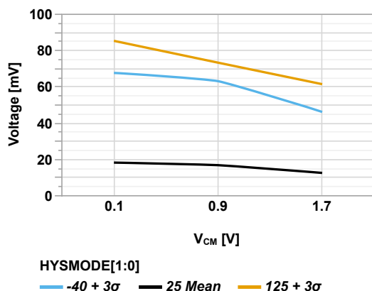
Figure 45-157. Input Hysteresis vs Common-Mode Voltage ( V_{DD} = 3.0V )
