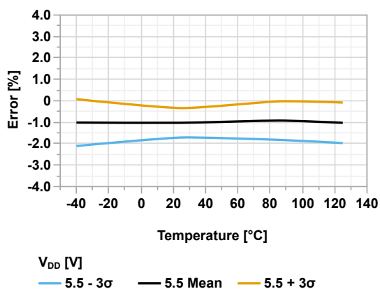
Figure 45-177. ADFVR Voltage Error vs Temperature ( V_{DD} = 5.5V , V_{REF} = 2.048V )
