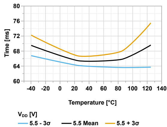
Figure 45-88. Start-Up Time vs Temperature (PWRTS = 'b10, V_{DD} = 5.5V )
