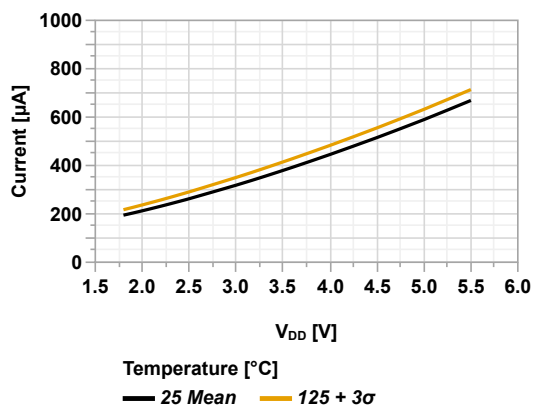
Figure 45-3. I_{DD} vs V_{DD} (HFINTOSC = 2 MHz, PMDx = 0x00)
