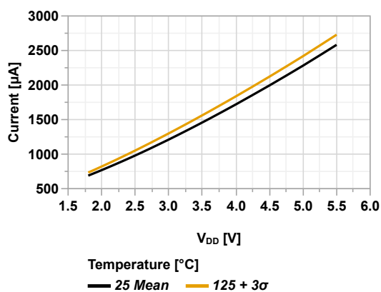
Figure 45-29. I_{DD} vs V_{DD} (Idle Mode, HFINTOSC = 16 MHz, PMDx = 0x00)
