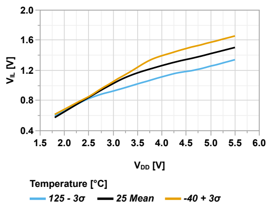
Figure 45-53. Input Pin with Schmitt Trigger Maximum V_{IL} vs V_{DD}
