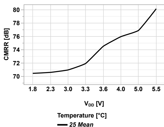
Figure 45-171. CMRR vs Common Mode Voltage ( V_{CM} = V_{DD} - 100\text{ mV} )
