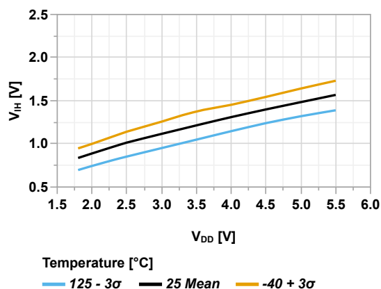
Figure 45-52. Input Pin with Schmitt Trigger Minimum V_{IH} vs V_{DD}
