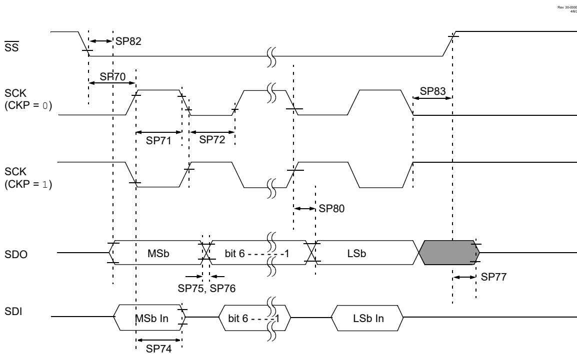
Figure 44-18. SPI Client Mode Timing (CKE = 1)
