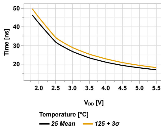
Figure 45-49. Fall Time vs V_{DD} (SLRxn = '0', T_A = 125^\circ\text{C} )
