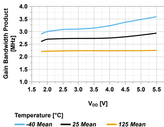
Figure 45-130. Gain Bandwidth Product vs V_{DD} (CPON = '1', GSEL = 'b001')
