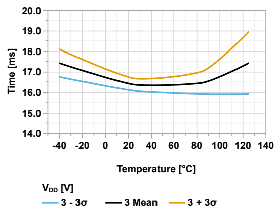
Figure 45-90. WDT Time-out Period vs Temperature ( V_{DD} = 3.0V )
