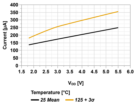
Figure 45-41. I_{PD} ADCRC (Converting) vs V_{DD}
