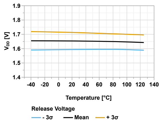
Figure 45-84. POR Release Voltage vs Temperature
