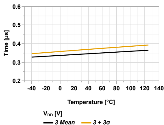
Figure 45-147. Turn-On Time vs Temperature ( V_{DD} = 3.0V, CPON = '0')
