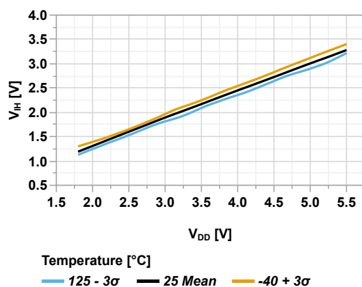
Figure 45-52. Input Pin with Schmitt Trigger Minimum V_{IH} vs V_{DD}
