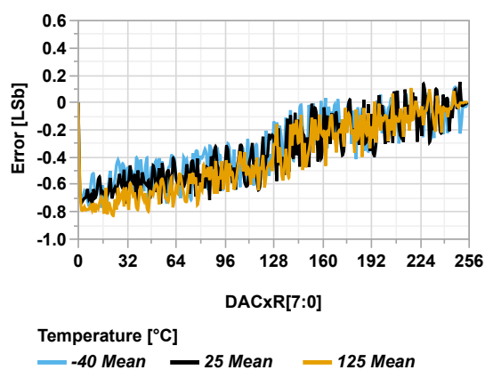
Figure 45-113. DAC INL vs. DAC Code ( V_{REF} = V_{DD} = 5.5V )
