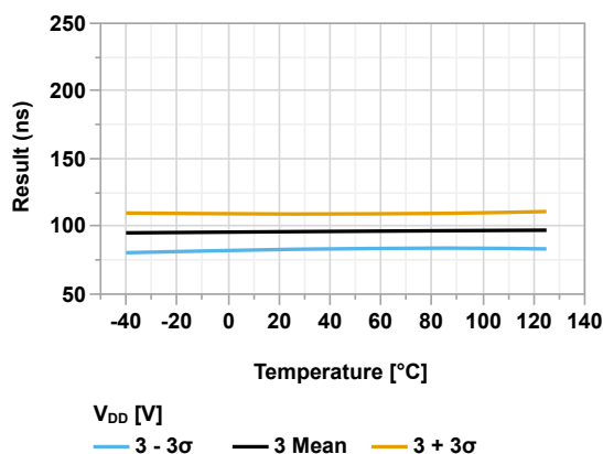
Figure 45-166. Rising Edge Response Time vs Temperature (CxSP = '0', CPON = 'b01', V_{DD} = 3.0V)
