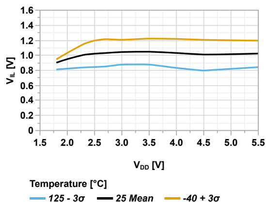
Figure 45-57. Input Pin with SMBus 3.0 Maximum V_{IL} vs V_{DD}
