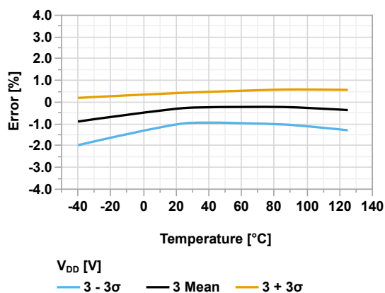
Figure 45-176. ADFVR Voltage Error vs Temperature ( V_{DD} = 3.0V , V_{REF} = 2.048V )
