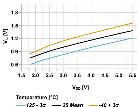
Figure 45-57. Input Pin with SMBus 3.0 Maximum V_{IL} vs V_{DD}
