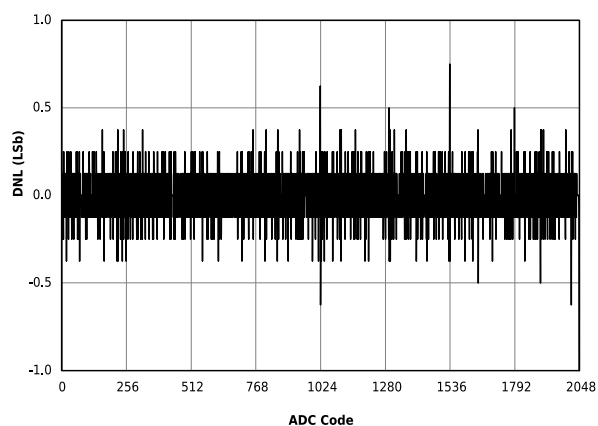
Figure 45-94. ADC DNL vs ADC Code (Single-Ended Mode, V_{REF+} = V_{DD} = 3.0V , T_{AD} = 1 \mu s )
