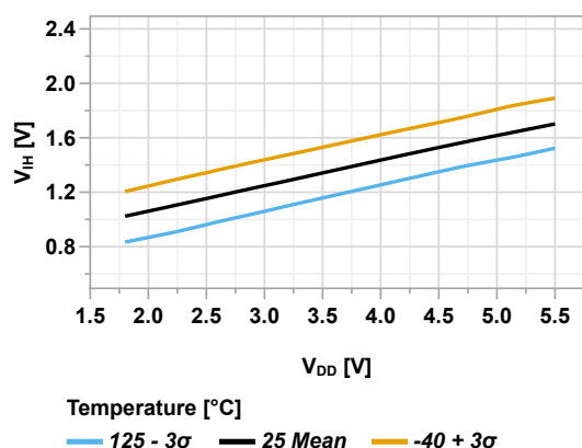
Figure 45-56. Input Pin with SMBus 3.0 Minimum V_{IH} vs V_{DD}
