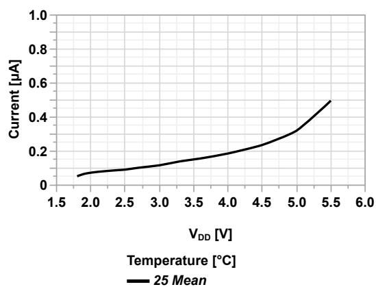
Figure 45-32. I_{PD} Base Typical
