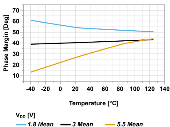
Figure 45-135. Phase Margin vs Temperature (CPON = '0', GSEL = 'b001')
