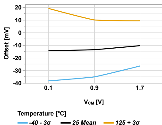
Figure 45-161. Input Offset vs Common-Mode Voltage ( V_{DD} = 3.0V )
