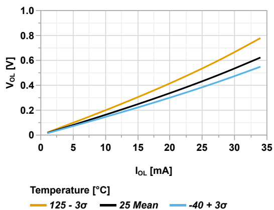
Figure 45-64. Output Pin Maximum V_{OL} vs Current ( V_{DD} = 3.0V )
