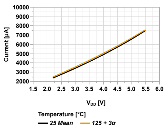
Figure 45-22. I_{DD} vs V_{DD} (ECL = 32 kHz, PMDx = 0xFF)
