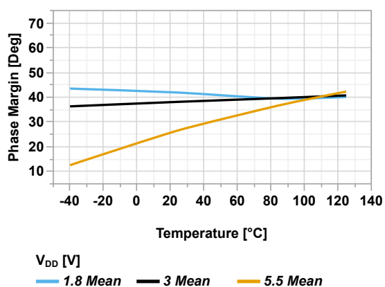
Figure 45-134. Phase Margin vs Temperature (CPON = '1', GSEL = 'b001')
