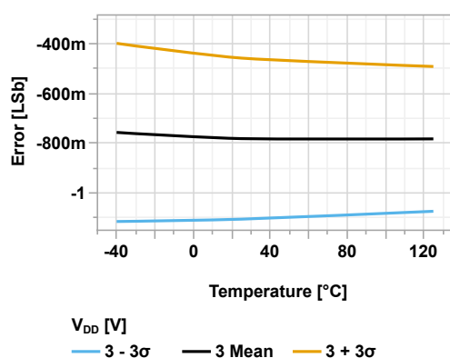
Figure 45-114. DAC INL vs. Temperature ( V_{REF} = V_{DD} = 3.0V )
