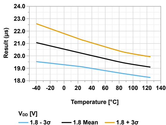
Figure 45-68. HFO Oscillator Start-Up Time vs Temperature ( V_{DD} = 1.8V )
