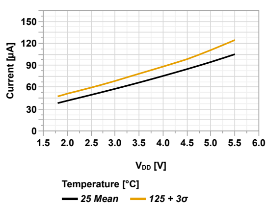
Figure 45-24. I_{DD} vs V_{DD} (ECL = 500 kHz, PMDx = 0xFF)
