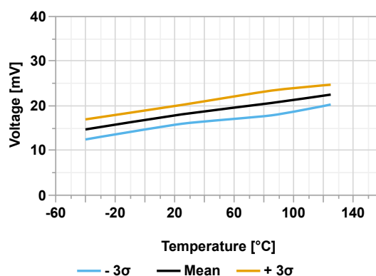
Figure 45-82. Low-Power Brown-out Reset Hysteresis vs Temperature
