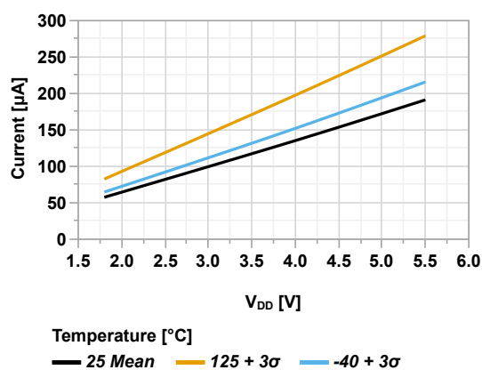
Figure 45-66. Weak Pull-Up Current vs V_{DD}
