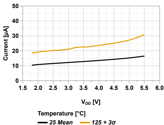
Figure 45-16. I_{DD} vs V_{DD} (XT = 1 MHz, PMDx = 0xFF)
