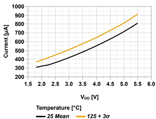
Figure 45-45. I_{PD} Op Amp (CPON = 'b11) vs V_{DD}
