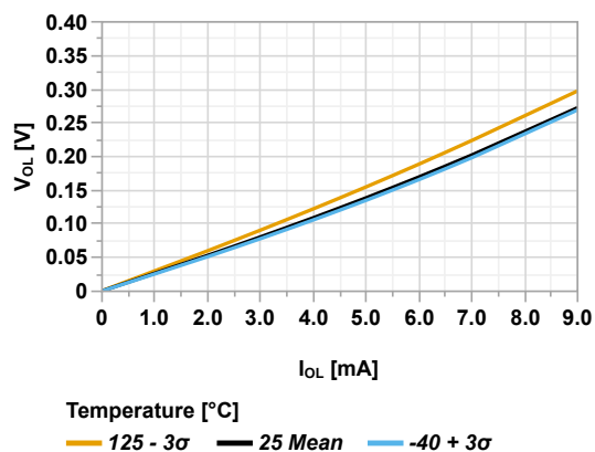
Figure 45-65. Output Pin Maximum V_{OL} vs Current ( V_{DD} = 5.5V )
