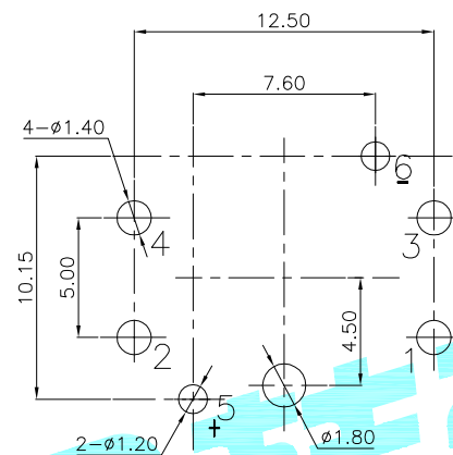
PCBLayout(pattern Side)
