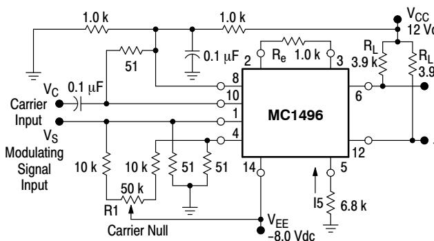
Figure 26. Balanced Modulator–Demodulator
