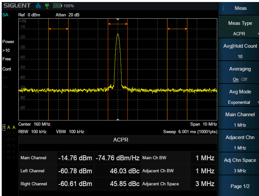
Figure 3-8 ACPR
