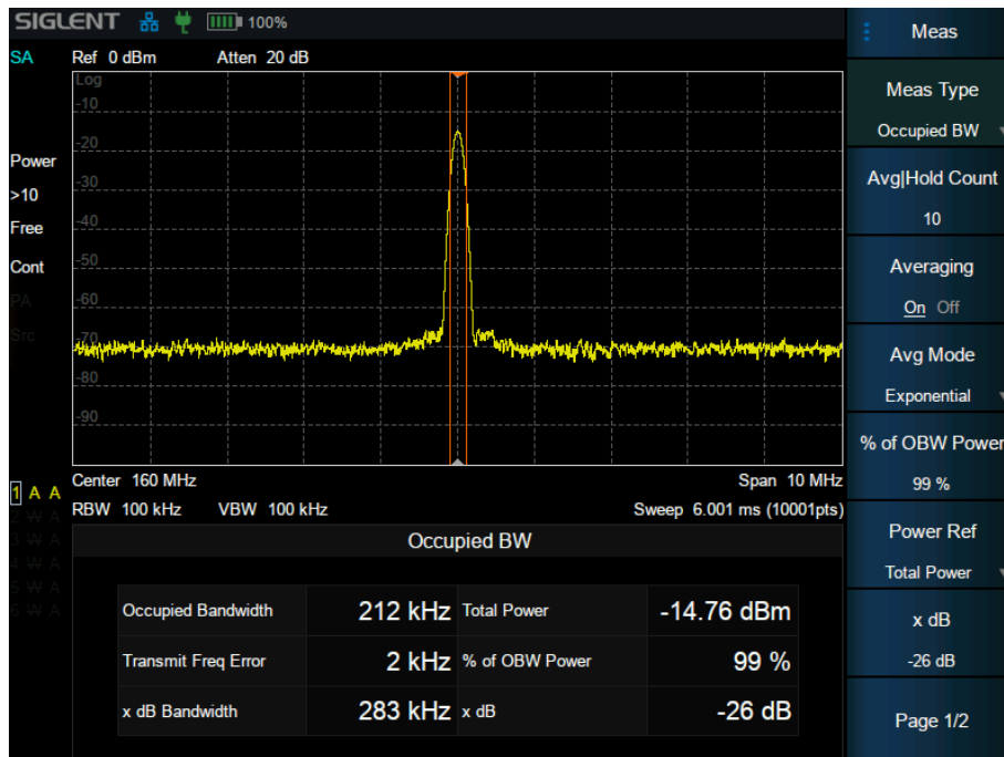
Figure 3-9 OBW
