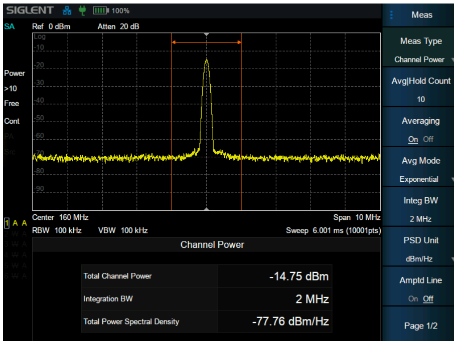
Figure 3-7 Channel Power
