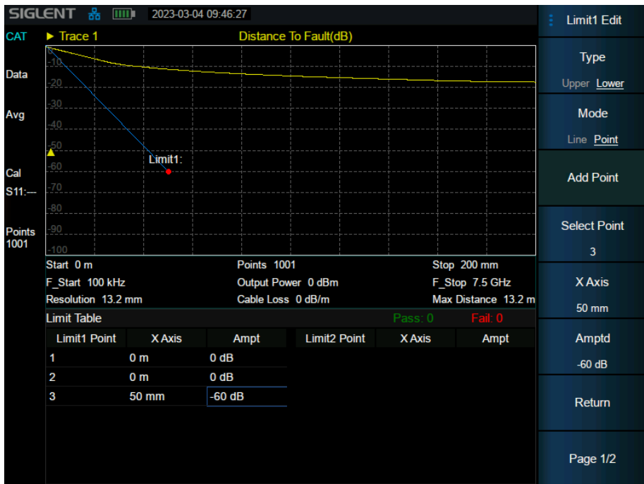
Figure 4-3 Limit Edit
