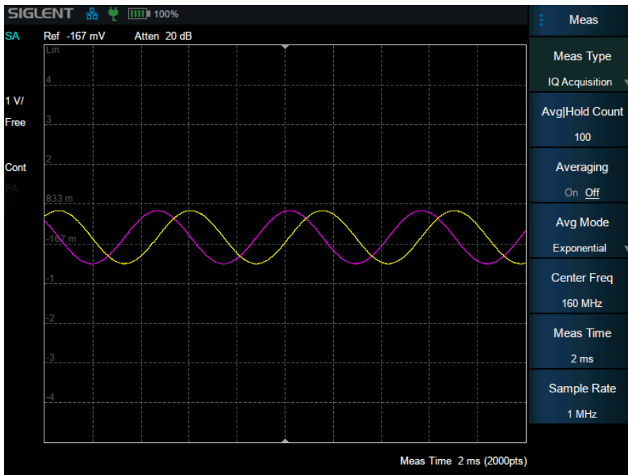
Figure 3-15 IQ Acquisition
