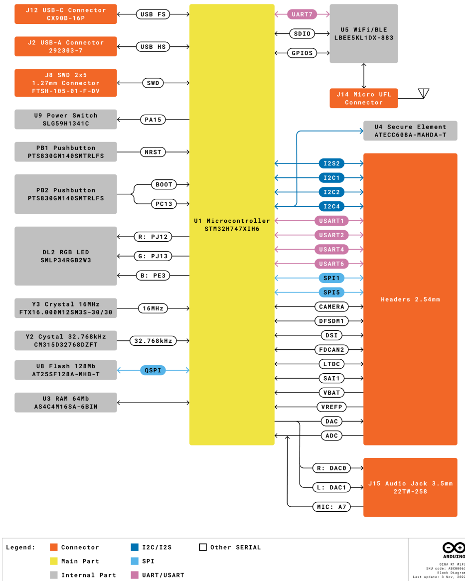
Arduino GIGA R1 WiFi Block Diagram
