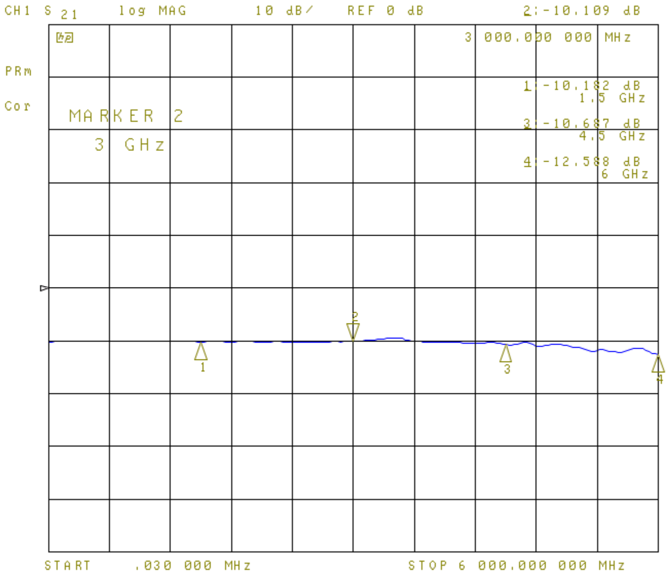
10dB Attenuator, S 21
