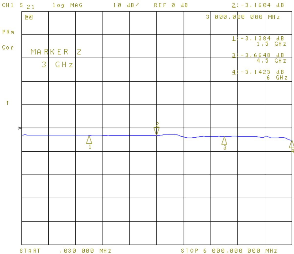
3dB Attenuator, S 21
