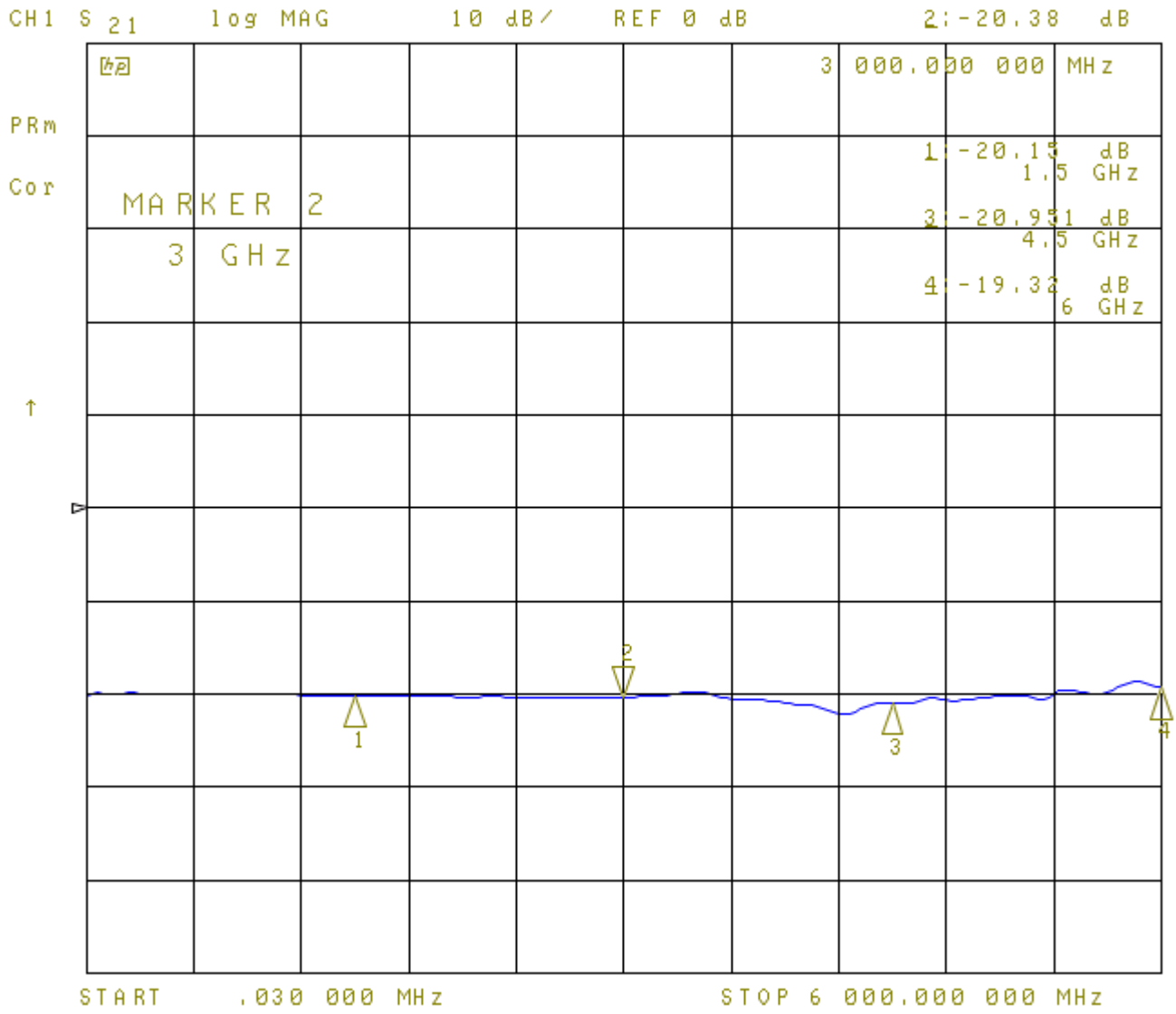
20dB Attenuator, S21
