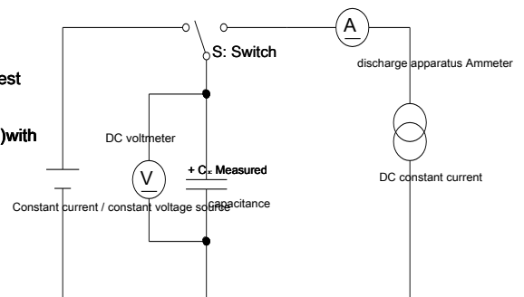
Map 1 Capacity test circuit
