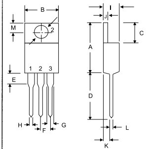
TO-220AB
