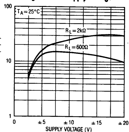
Voltage Gain vs Supply Voltage
