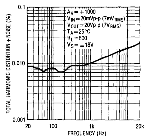
THD + Noise vs Frequency ( A_V = +1000 )
