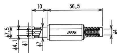
No.MP-139SF DC PLUG(7.5×4.1 Center Pin : 1 φ mm) FOR COMPUTER GAME
