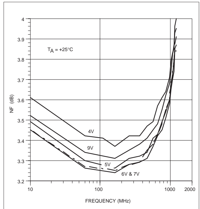
Figure 23. Noise Figure vs Frequency and VCC in a 50Ω System
