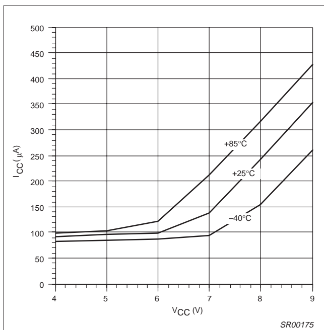
Figure 9. Disabled Supply Current vs Vcc and Temperature
