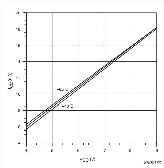
Figure 8. Supply Current vs Supply Voltage and Temperature
