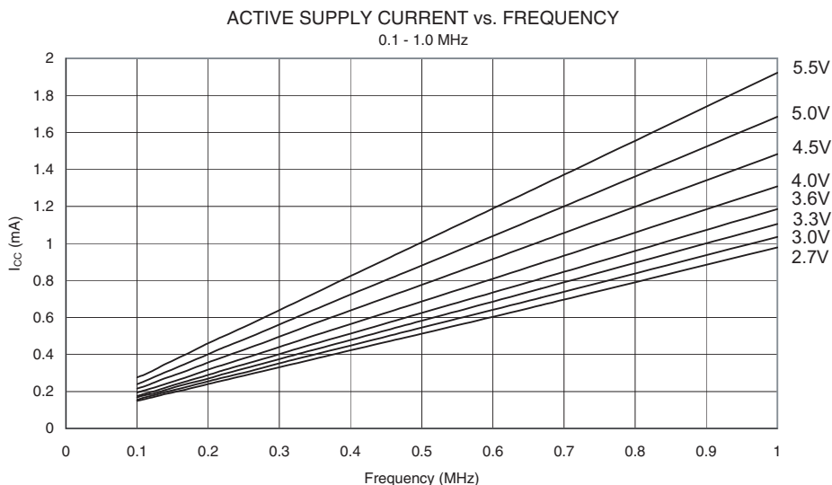
Figure 148. Active Supply Current vs. Frequency (0.1 - 1.0 MHz)
