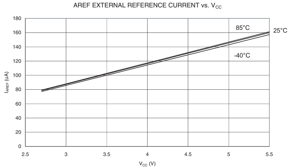
Figure 207. Aref External Reference Current vs. V_{CC}
