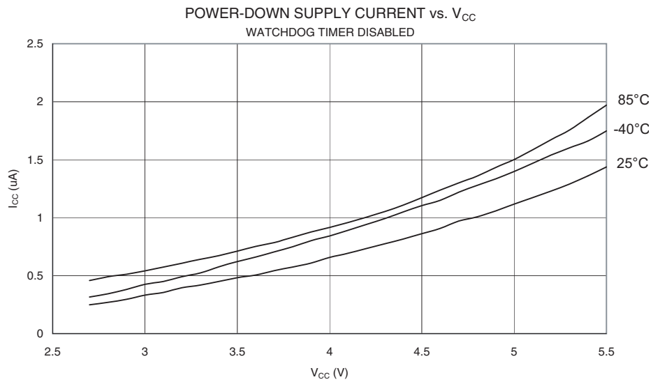
Figure 162. Power-Down Supply Current vs. V_{CC} (Watchdog Timer Disabled)
