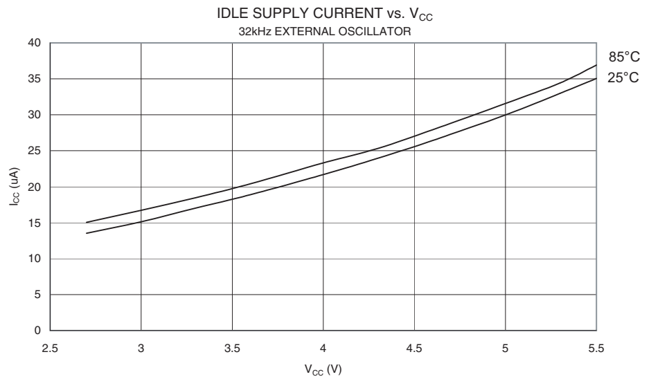
Figure 161. Idle Supply Current vs. V_{CC} (32 kHz External Oscillator)
