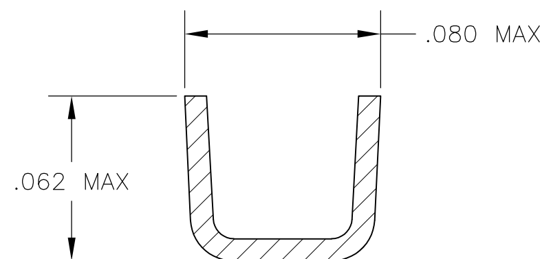
SECTION A—A SCALE 20:1
