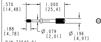
P/N 73542-01 SHORT THUMB SCREW
