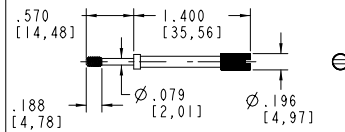
P/N 73542-04 LONG THUMB SCREW
