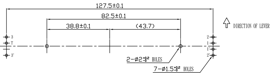
MOUNTING HOLE DETAIL
