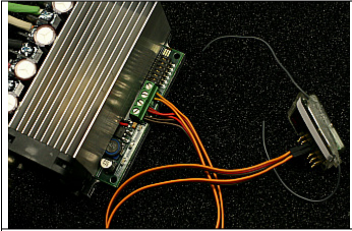
Figure 5.1: R/C connection
