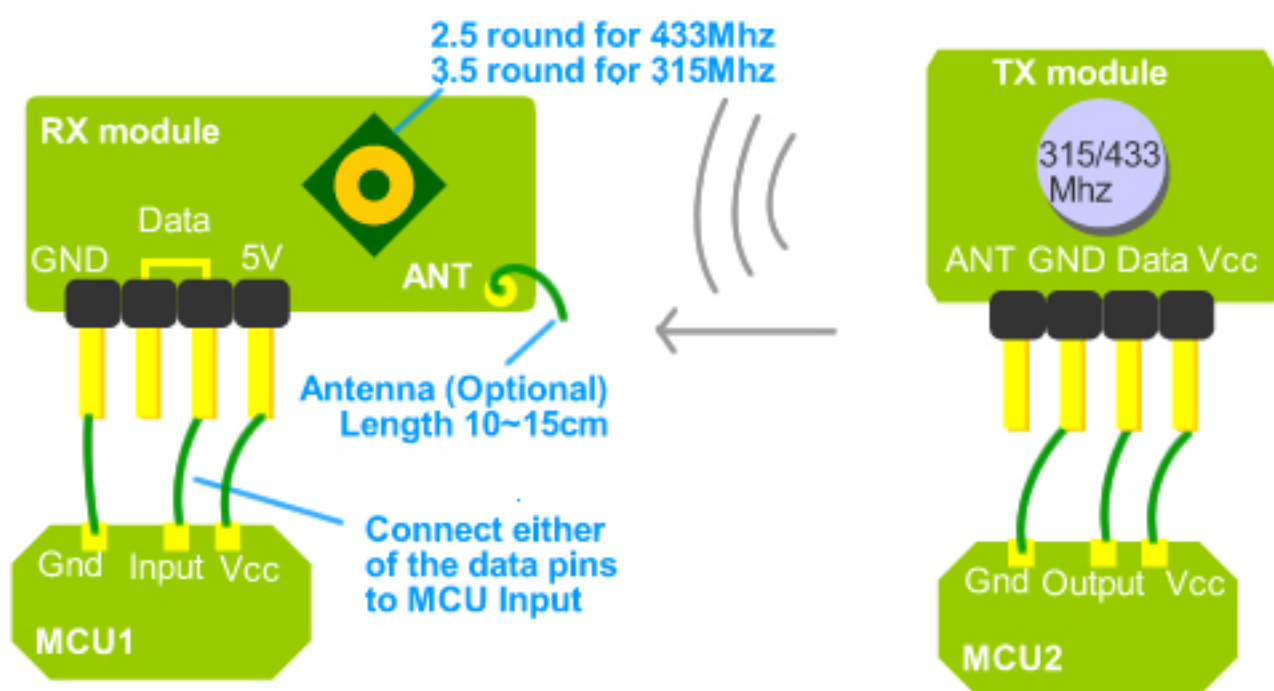
Demostration scheme of 433/315Mhz RF kit
