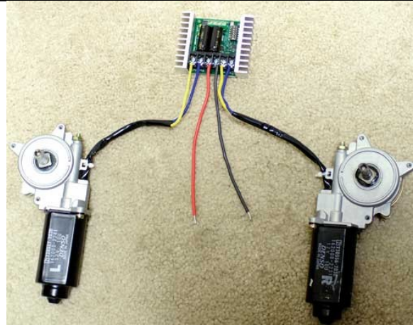
The motors connect to terminals M1A/B and M2A/B
