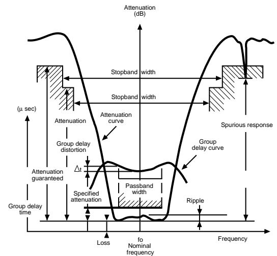
Figure 3) MCF Characteristics Curve
