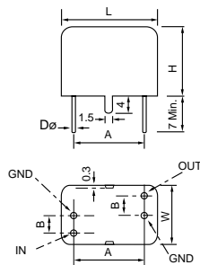
Figure 4) SC Pkg with Dimensional Chart
