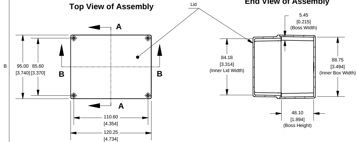
SECTION A-A End View of Assembly
