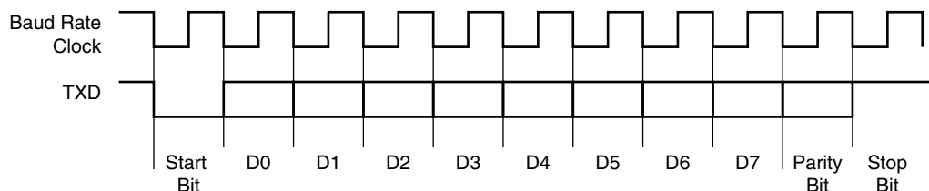
Figure 31-8. Character Transmit
