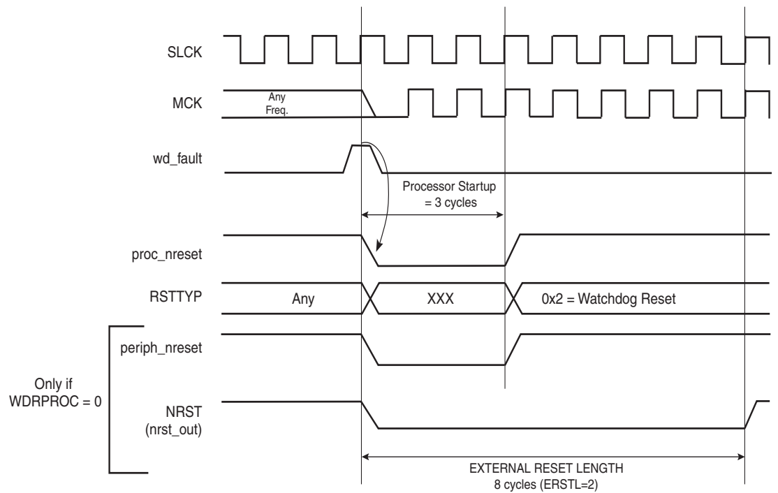
Figure 13-8. Watchdog Reset
