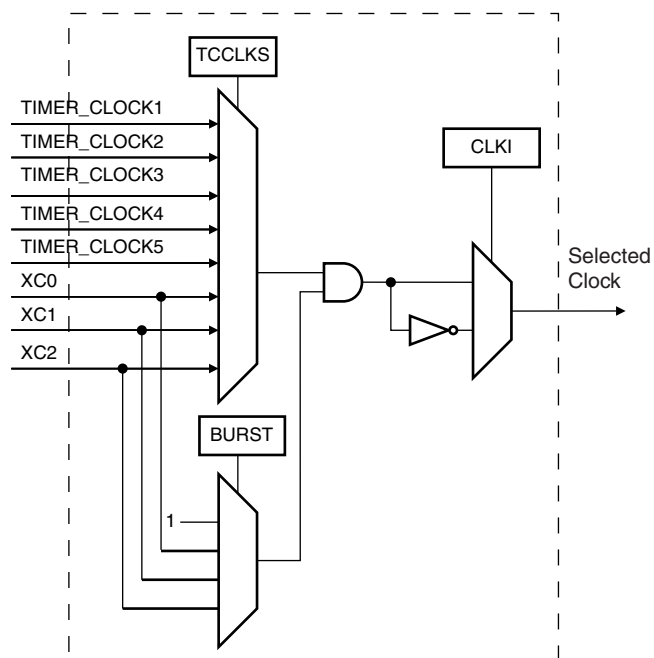
Figure 33-3. Clock Selection
