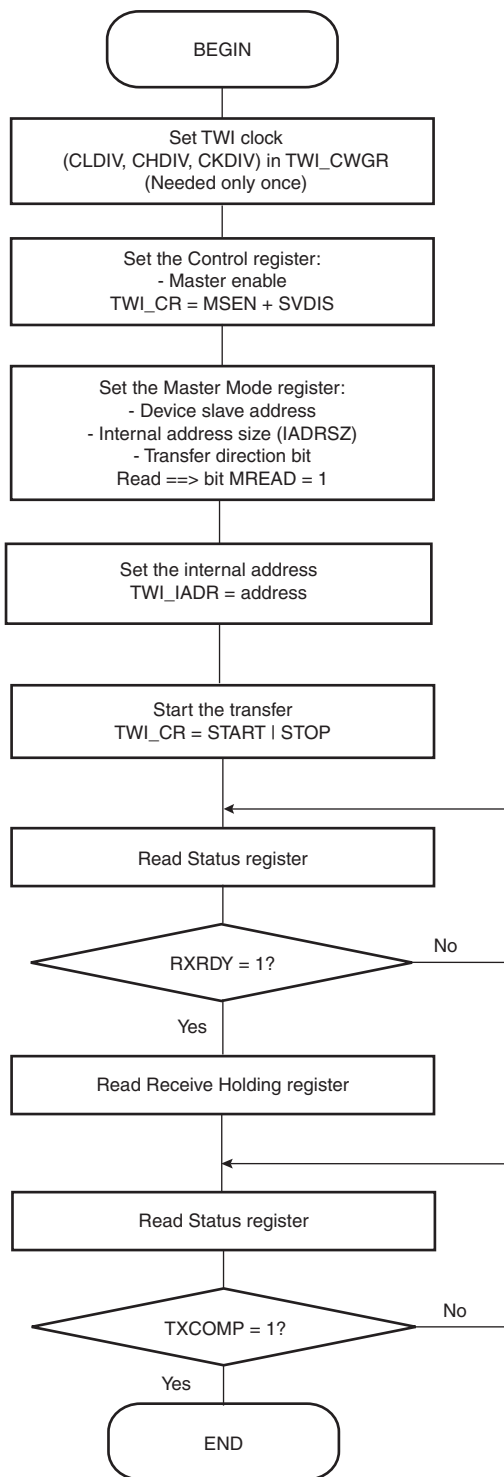
Figure 30-18. TWI Read Operation with Single Data Byte and Internal Address
