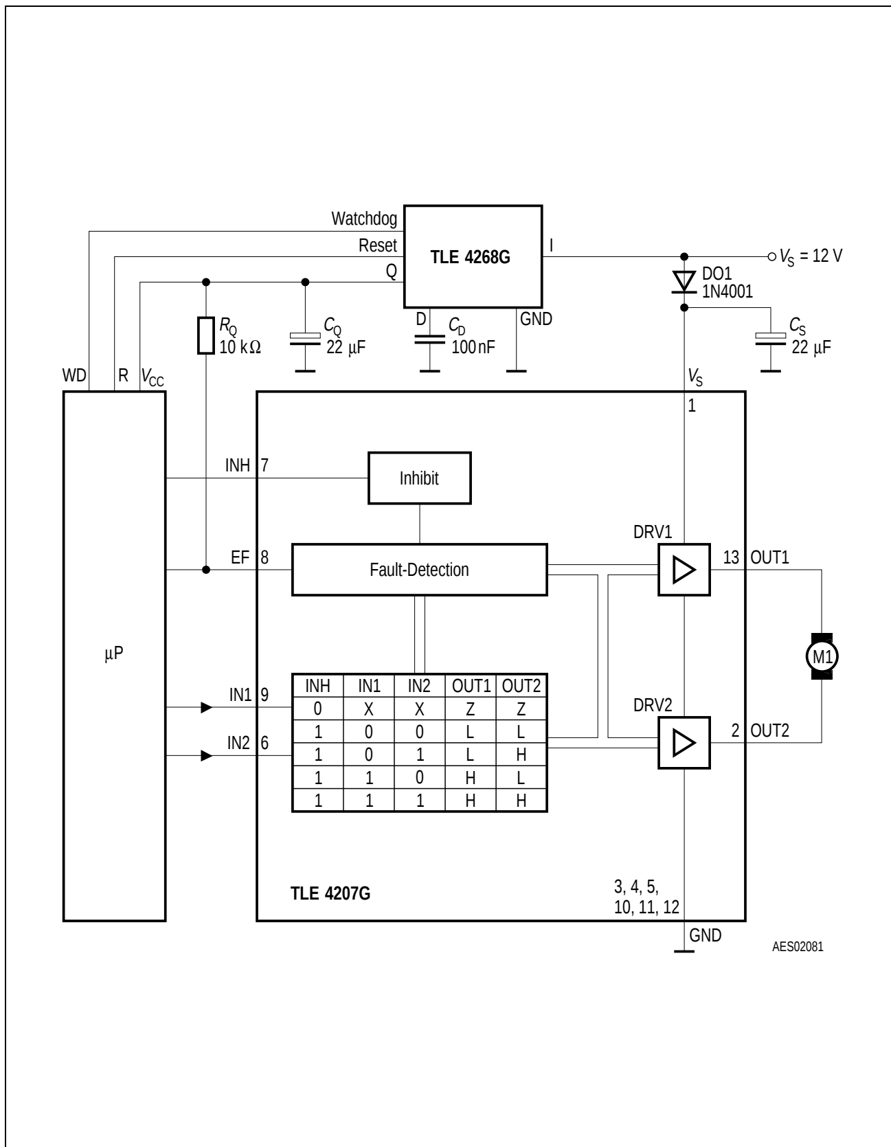
Figure 3 Application Circuit
