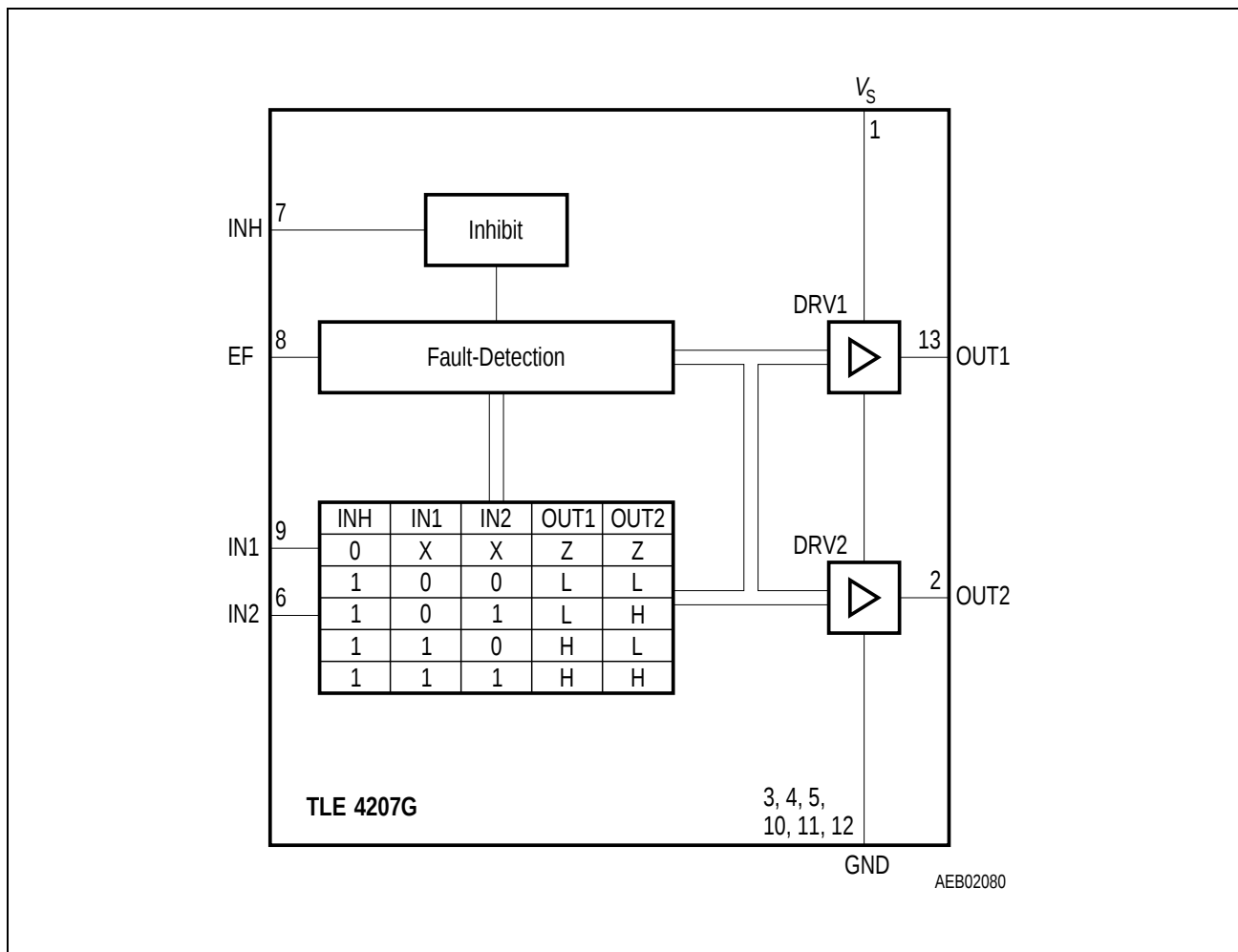
Figure 2 Block Diagram
