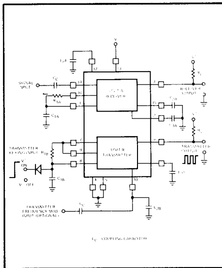
Figure 14. Tone Transceiver
