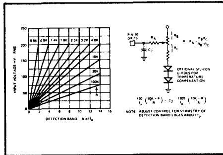
Figure 10. Bandwidth Reduction
