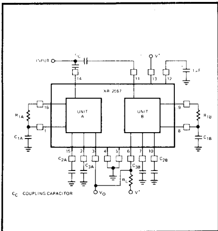
Figure 13. Wide-Band Tone Detection
