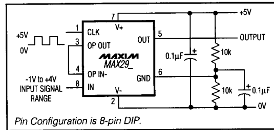
Figure 3. +5V Single-Supply Operation
