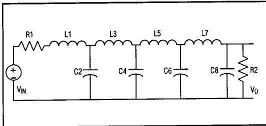
Figure 2. 8th-Order Ladder Filter Network
