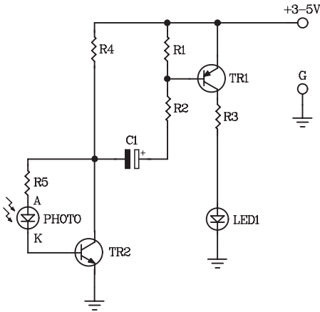
Figure 2. The infrared remote checker circuit
