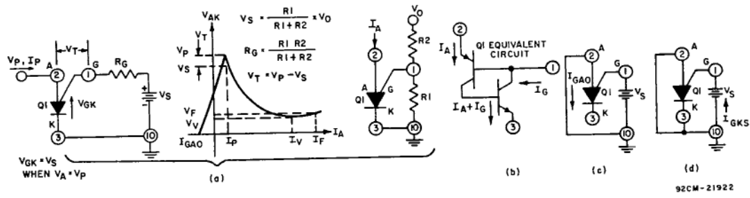
Fig. 22 - General anode characteristics for Q1 (PUT).
