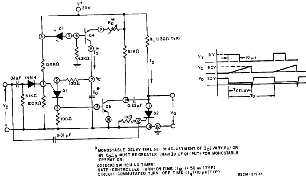
Fig. 33 - Monostable multivibrator with variable delay.
