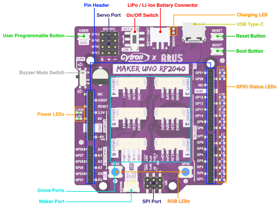
Figure 1: MAKER-UNO-RP2040 Board Functions (TOP)
