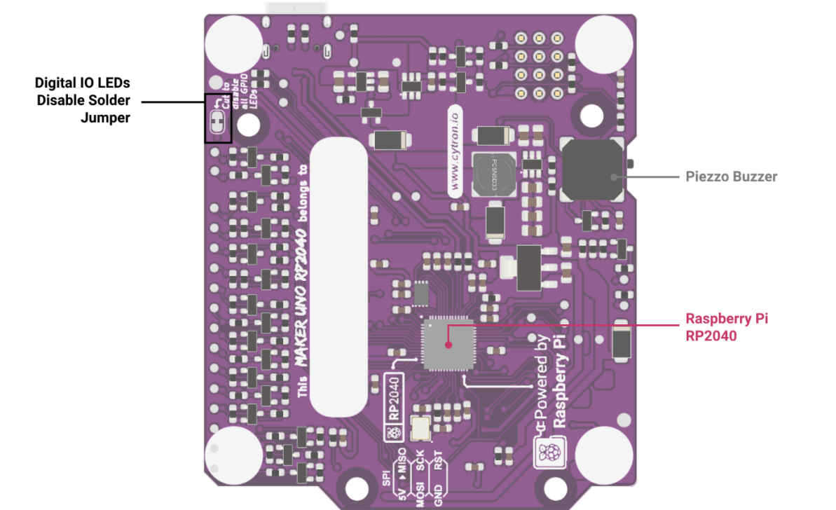
Figure 2: MAKER-UNO-RP2040 Board Functions (Bottom)
